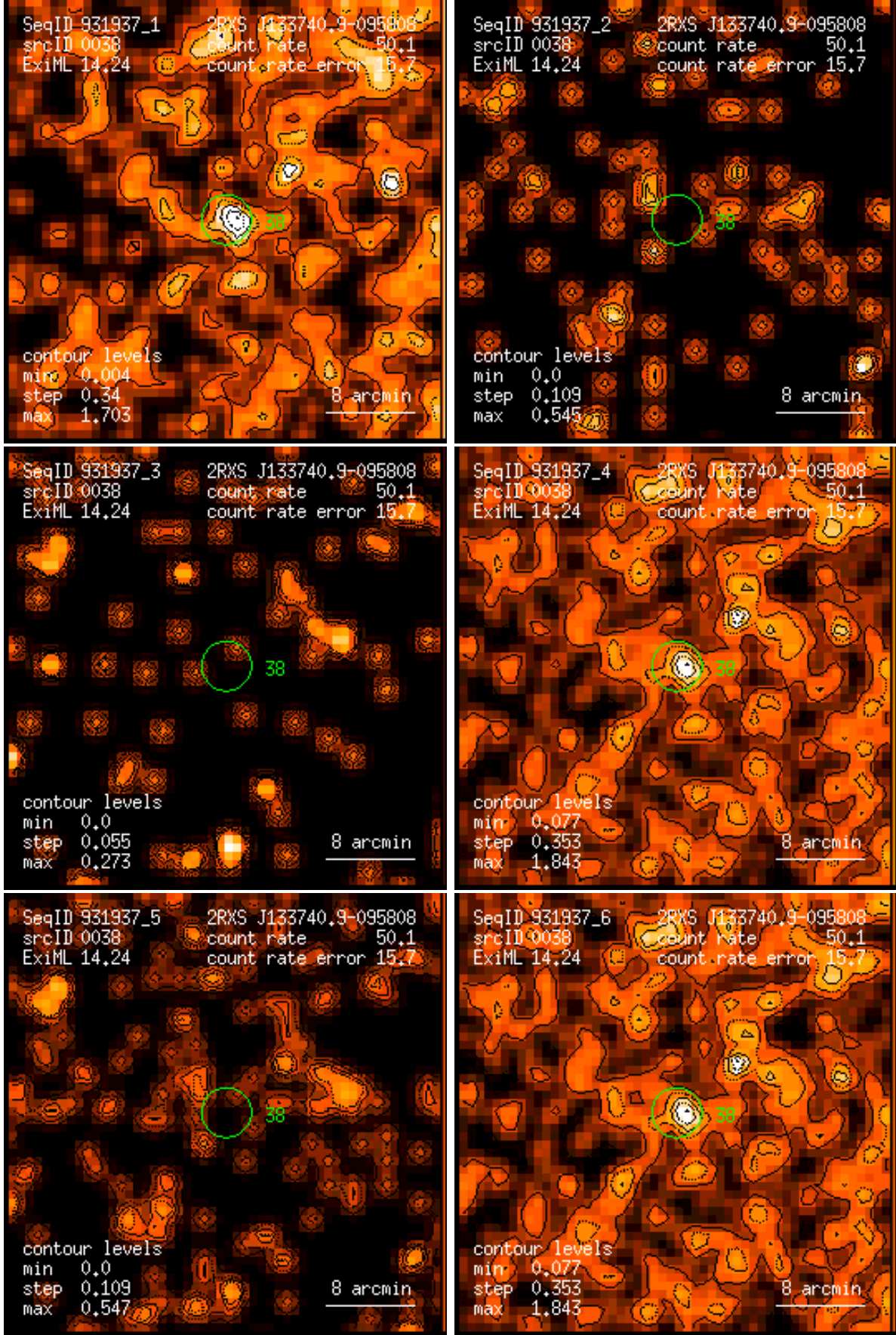
Figure 38: RASS 931937: detection 0038: band rate images, Gaussian filter: (1) PSPC channels 11 – 41, (2) 52 – 90, (3) 91 – 201, (4) 11 – 235, (5) 52 – 201, (6) 11 – 201. Broad band rates in counts/ks. Band rate contour levels in counts/ks/arcmin 2 .
