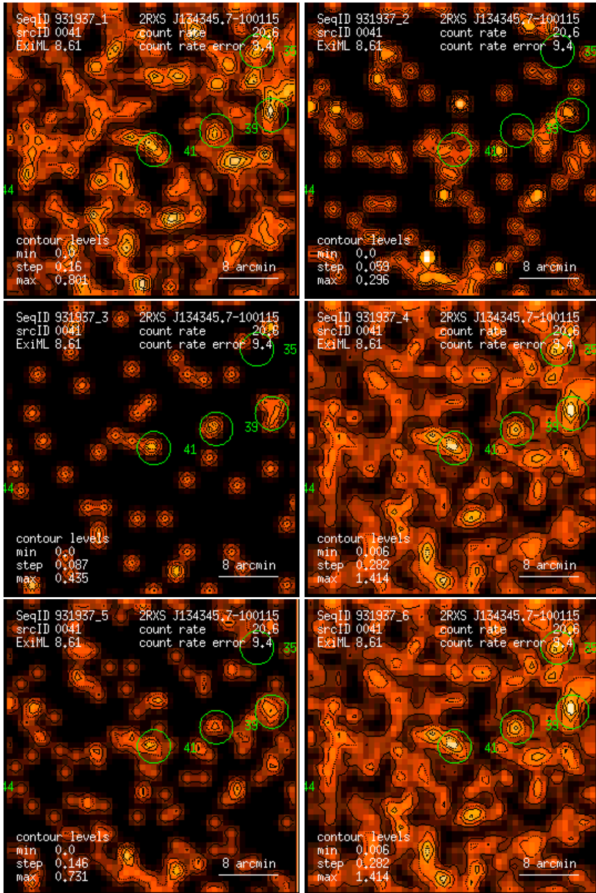
Figure 41: RASS 931937: detection 0041: band rate images, Gaussian filter: (1) PSPC channels 11 – 41, (2) 52 – 90, (3) 91 – 201, (4) 11 – 235, (5) 52 – 201, (6) 11 – 201. Broad band rates in counts/ks. Band rate contour levels in counts/ks/arcmin 2 .
