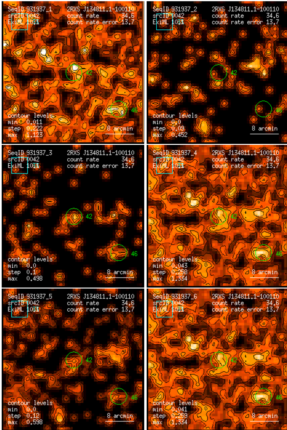
Figure 42: RASS 931937: detection 0042: band rate images, Gaussian filter: (1) PSPC channels 11 – 41, (2) 52 – 90, (3) 91 – 201, (4) 11 – 235, (5) 52 – 201, (6) 11 – 201. Broad band rates in counts/ks. Band rate contour levels in counts/ks/arcmin 2 .
