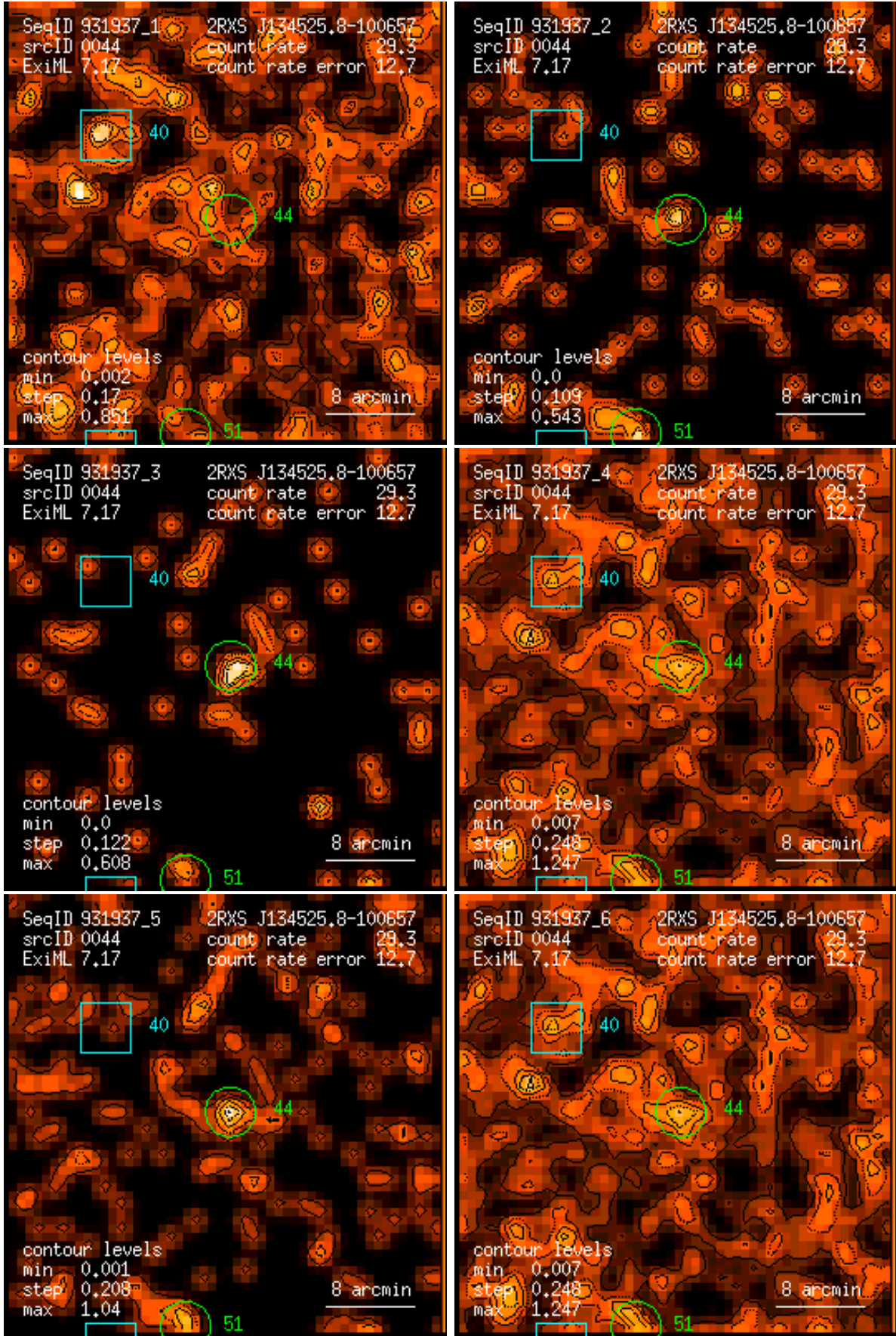
Figure 44: RASS 931937: detection 0044: band rate images, Gaussian filter: (1) PSPC channels 11 – 41, (2) 52 – 90, (3) 91 – 201, (4) 11 – 235, (5) 52 – 201, (6) 11 – 201. Broad band rates in counts/ks. Band rate contour levels in counts/ks/arcmin 2 .
