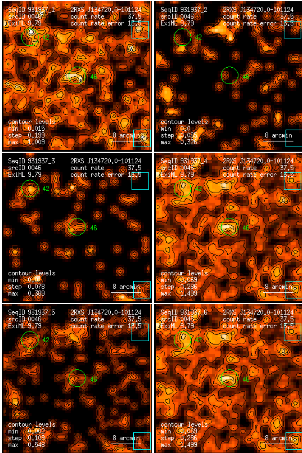
Figure 46: RASS 931937: detection 0046: band rate images, Gaussian filter: (1) PSPC channels 11 – 41, (2) 52 – 90, (3) 91 – 201, (4) 11 – 235, (5) 52 – 201, (6) 11 – 201. Broad band rates in counts/ks. Band rate contour levels in counts/ks/arcmin 2 .
