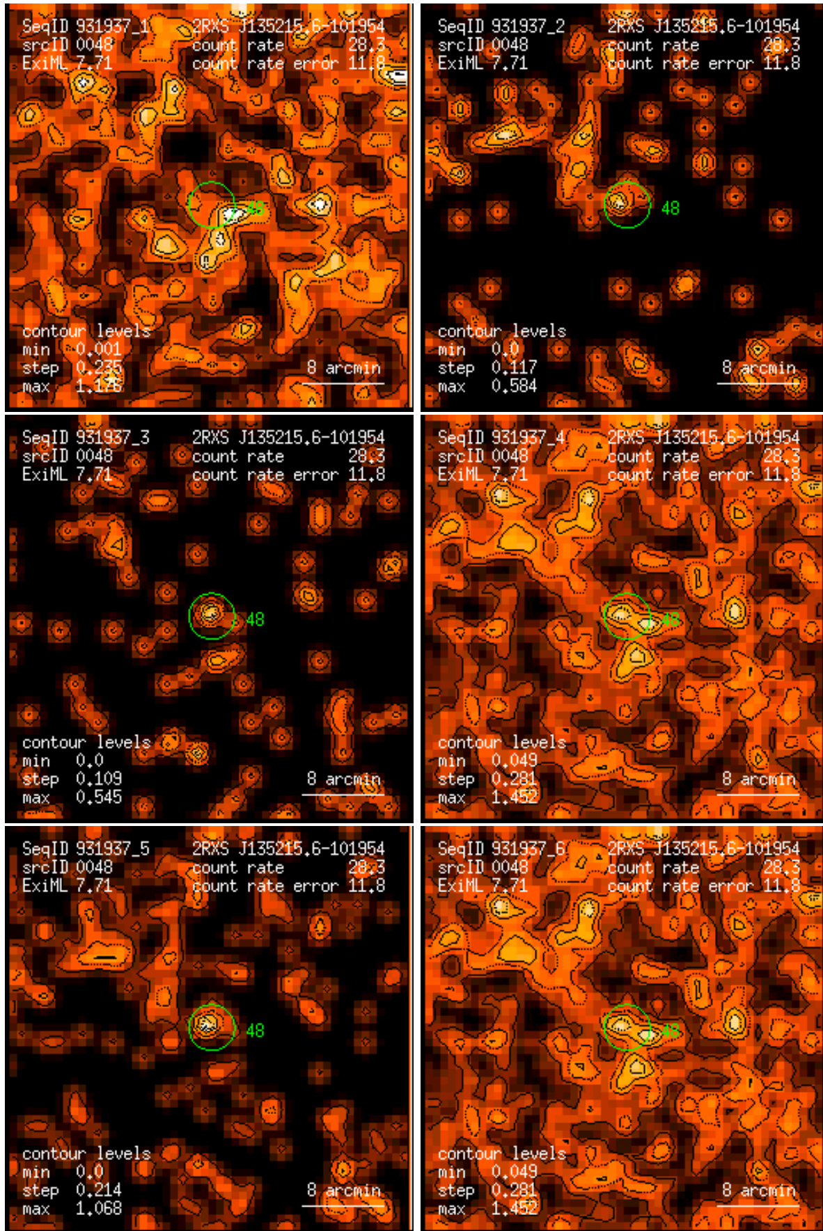
Figure 48: RASS 931937: detection 0048: band rate images, Gaussian filter: (1) PSPC channels 11 – 41, (2) 52 – 90, (3) 91 – 201, (4) 11 – 235, (5) 52 – 201, (6) 11 – 201. Broad band rates in counts/ks. Band rate contour levels in counts/ks/arcmin 2 .
