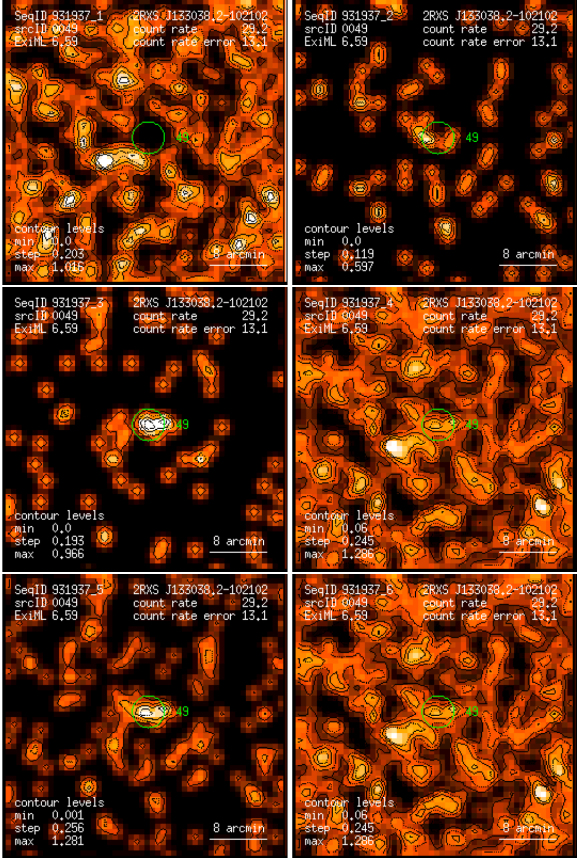
Figure 49: RASS 931937: detection 0049: band rate images, Gaussian filter: (1) PSPC channels 11 – 41, (2) 52 – 90, (3) 91 – 201, (4) 11 – 235, (5) 52 – 201, (6) 11 – 201. Broad band rates in counts/ks. Band rate contour levels in counts/ks/arcmin 2 .
