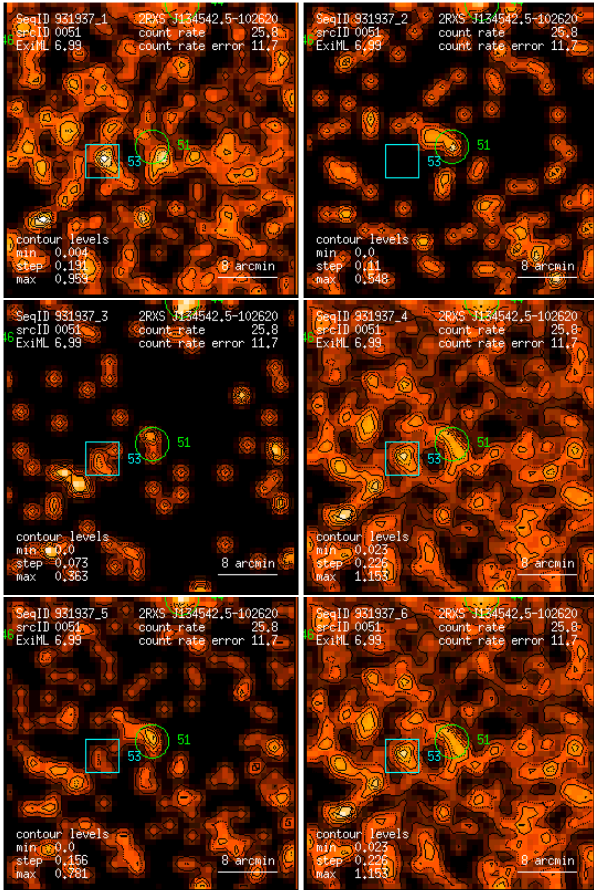
Figure 51: RASS 931937: detection 0051: band rate images, Gaussian filter: (1) PSPC channels 11 – 41, (2) 52 – 90, (3) 91 – 201, (4) 11 – 235, (5) 52 – 201, (6) 11 – 201. Broad band rates in counts/ks. Band rate contour levels in counts/ks/arcmin 2 .
