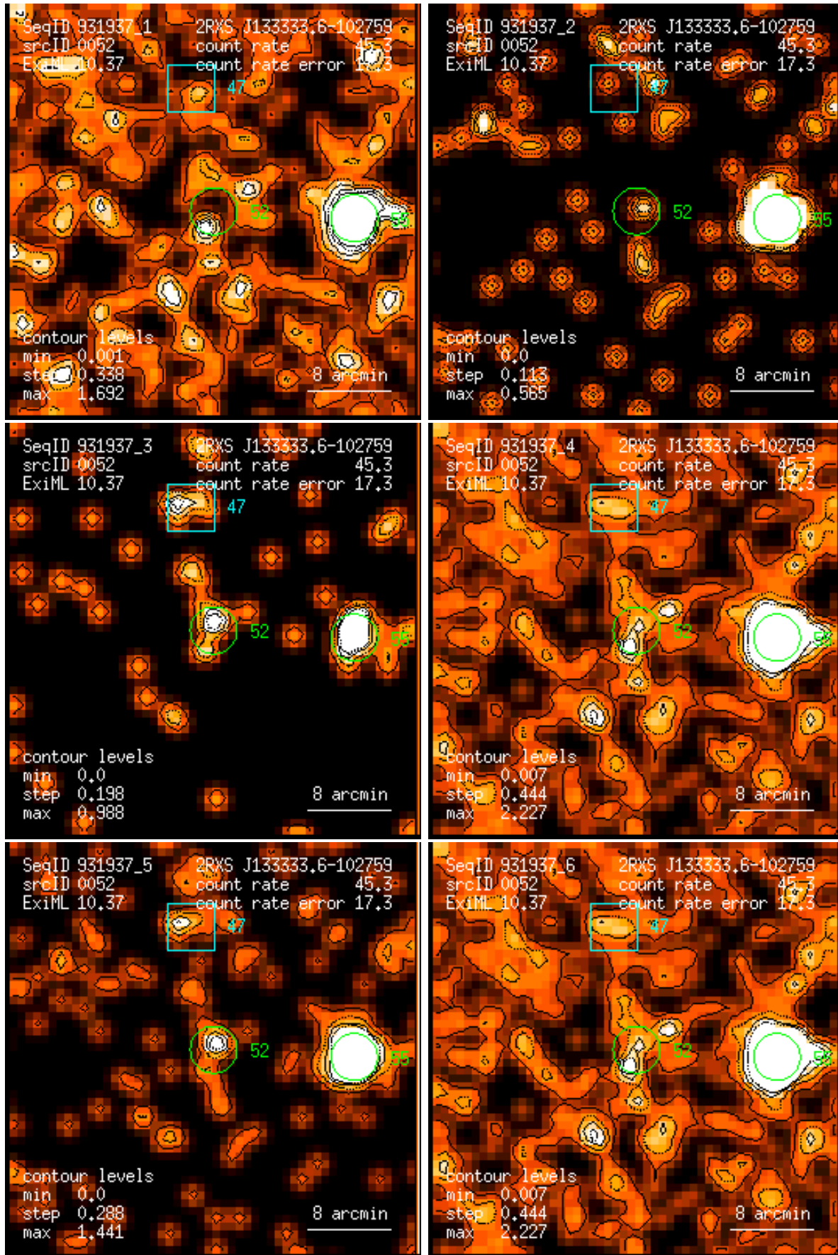
Figure 52: RASS 931937: detection 0052: band rate images, Gaussian filter: (1) PSPC channels 11 – 41, (2) 52 – 90, (3) 91 – 201, (4) 11 – 235, (5) 52 – 201, (6) 11 – 201. Broad band rates in counts/ks. Band rate contour levels in counts/ks/arcmin 2 .
