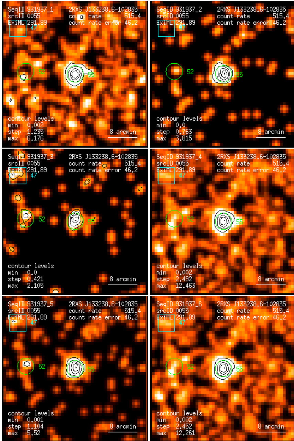
Figure 55: RASS 931937: detection 0055: band rate images, Gaussian filter: (1) PSPC channels 11 – 41, (2) 52 – 90, (3) 91 – 201, (4) 11 – 235, (5) 52 – 201, (6) 11 – 201. Broad band rates in counts/ks. Band rate contour levels in counts/ks/arcmin 2 .
