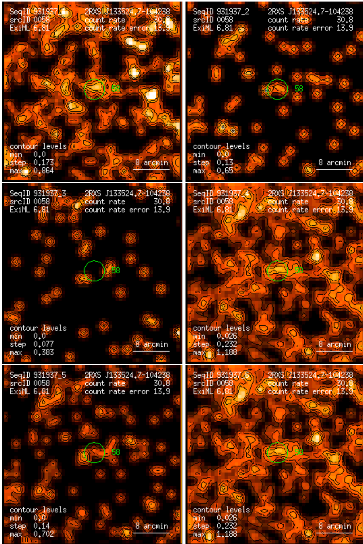
Figure 58: RASS 931937: detection 0058: band rate images, Gaussian filter: (1) PSPC channels 11 – 41, (2) 52 – 90, (3) 91 – 201, (4) 11 – 235, (5) 52 – 201, (6) 11 – 201. Broad band rates in counts/ks. Band rate contour levels in counts/ks/arcmin 2 .
