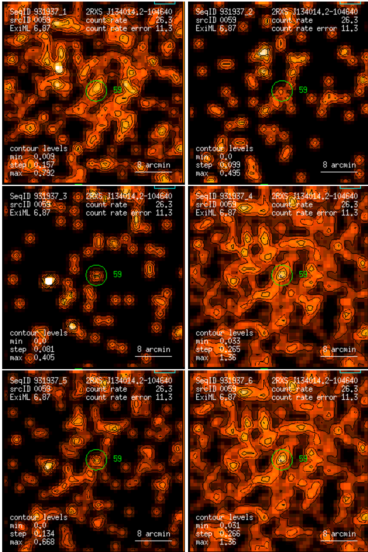
Figure 59: RASS 931937: detection 0059: band rate images, Gaussian filter: (1) PSPC channels 11 – 41, (2) 52 – 90, (3) 91 – 201, (4) 11 – 235, (5) 52 – 201, (6) 11 – 201. Broad band rates in counts/ks. Band rate contour levels in counts/ks/arcmin 2 .
