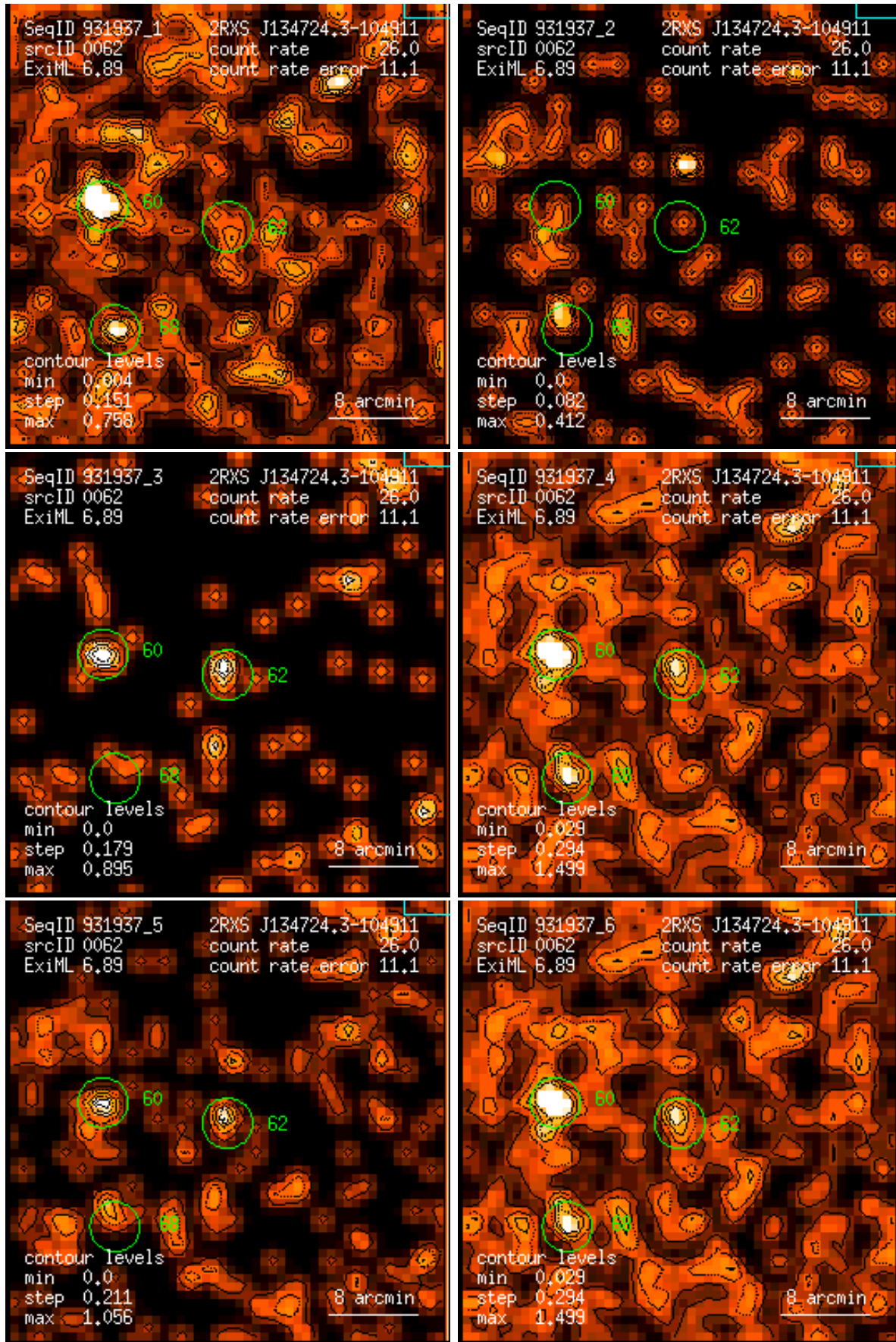
Figure 62: RASS 931937: detection 0062: band rate images, Gaussian filter: (1) PSPC channels 11 – 41, (2) 52 – 90, (3) 91 – 201, (4) 11 – 235, (5) 52 – 201, (6) 11 – 201. Broad band rates in counts/ks. Band rate contour levels in counts/ks/arcmin 2 .
