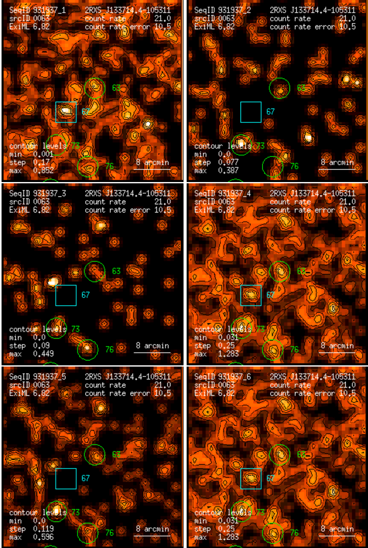
Figure 63: RASS 931937: detection 0063: band rate images, Gaussian filter: (1) PSPC channels 11 – 41, (2) 52 – 90, (3) 91 – 201, (4) 11 – 235, (5) 52 – 201, (6) 11 – 201. Broad band rates in counts/ks. Band rate contour levels in counts/ks/arcmin 2 .
