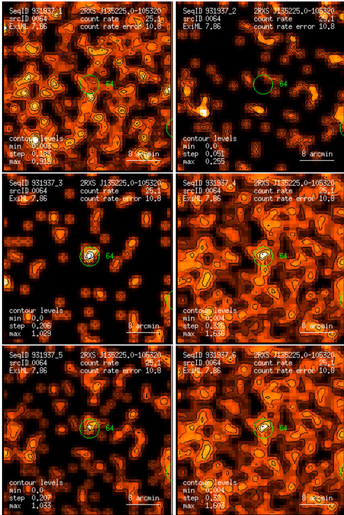
Figure 64: RASS 931937: detection 0064: band rate images, Gaussian filter: (1) PSPC channels 11 – 41, (2) 52 – 90, (3) 91 – 201, (4) 11 – 235, (5) 52 – 201, (6) 11 – 201. Broad band rates in counts/ks. Band rate contour levels in counts/ks/arcmin 2 .
