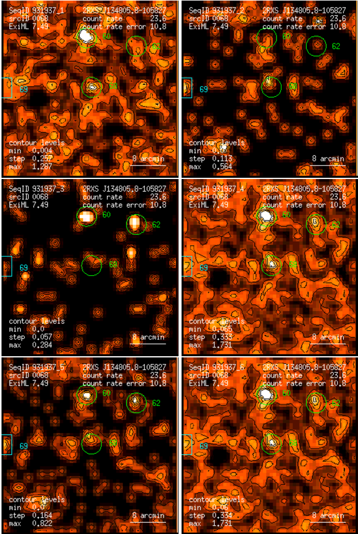
Figure 68: RASS 931937: detection 0068: band rate images, Gaussian filter: (1) PSPC channels 11 – 41, (2) 52 – 90, (3) 91 – 201, (4) 11 – 235, (5) 52 – 201, (6) 11 – 201. Broad band rates in counts/ks. Band rate contour levels in counts/ks/arcmin 2 .
