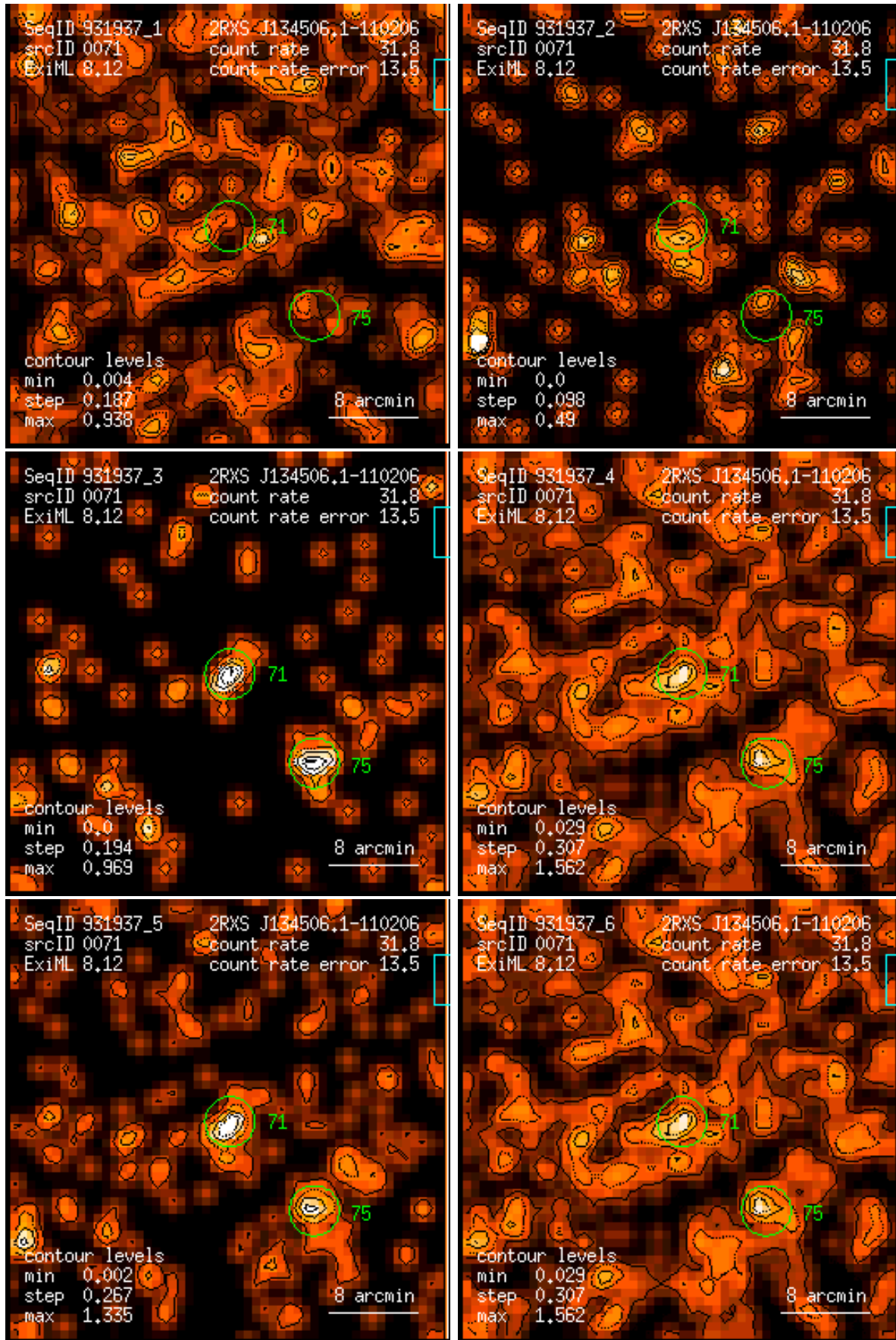
Figure 71: RASS 931937: detection 0071: band rate images, Gaussian filter: (1) PSPC channels 11 – 41, (2) 52 – 90, (3) 91 – 201, (4) 11 – 235, (5) 52 – 201, (6) 11 – 201. Broad band rates in counts/ks. Band rate contour levels in counts/ks/arcmin 2 .
