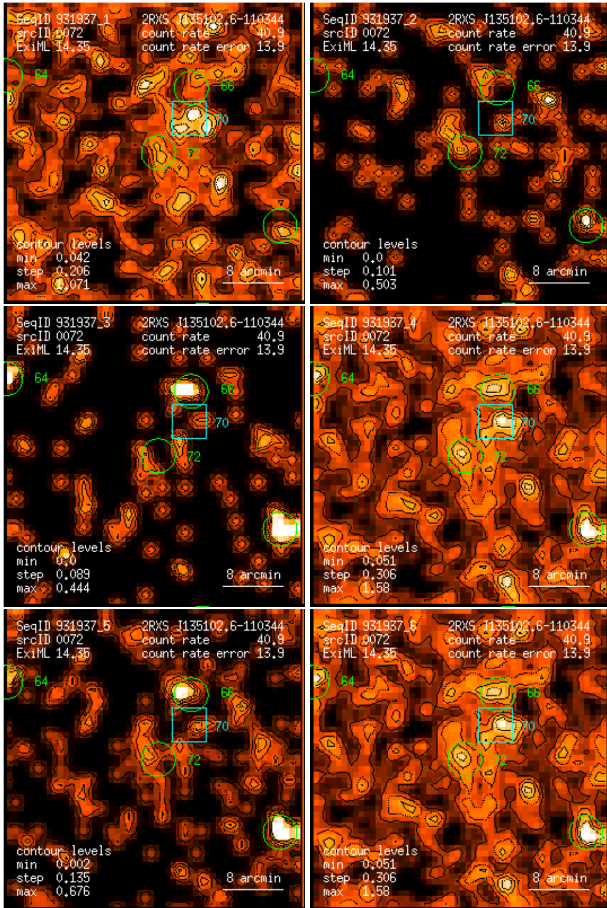
Figure 72: RASS 931937: detection 0072: band rate images, Gaussian filter: (1) PSPC channels 11 – 41, (2) 52 – 90, (3) 91 – 201, (4) 11 – 235, (5) 52 – 201, (6) 11 – 201. Broad band rates in counts/ks. Band rate contour levels in counts/ks/arcmin 2 .
