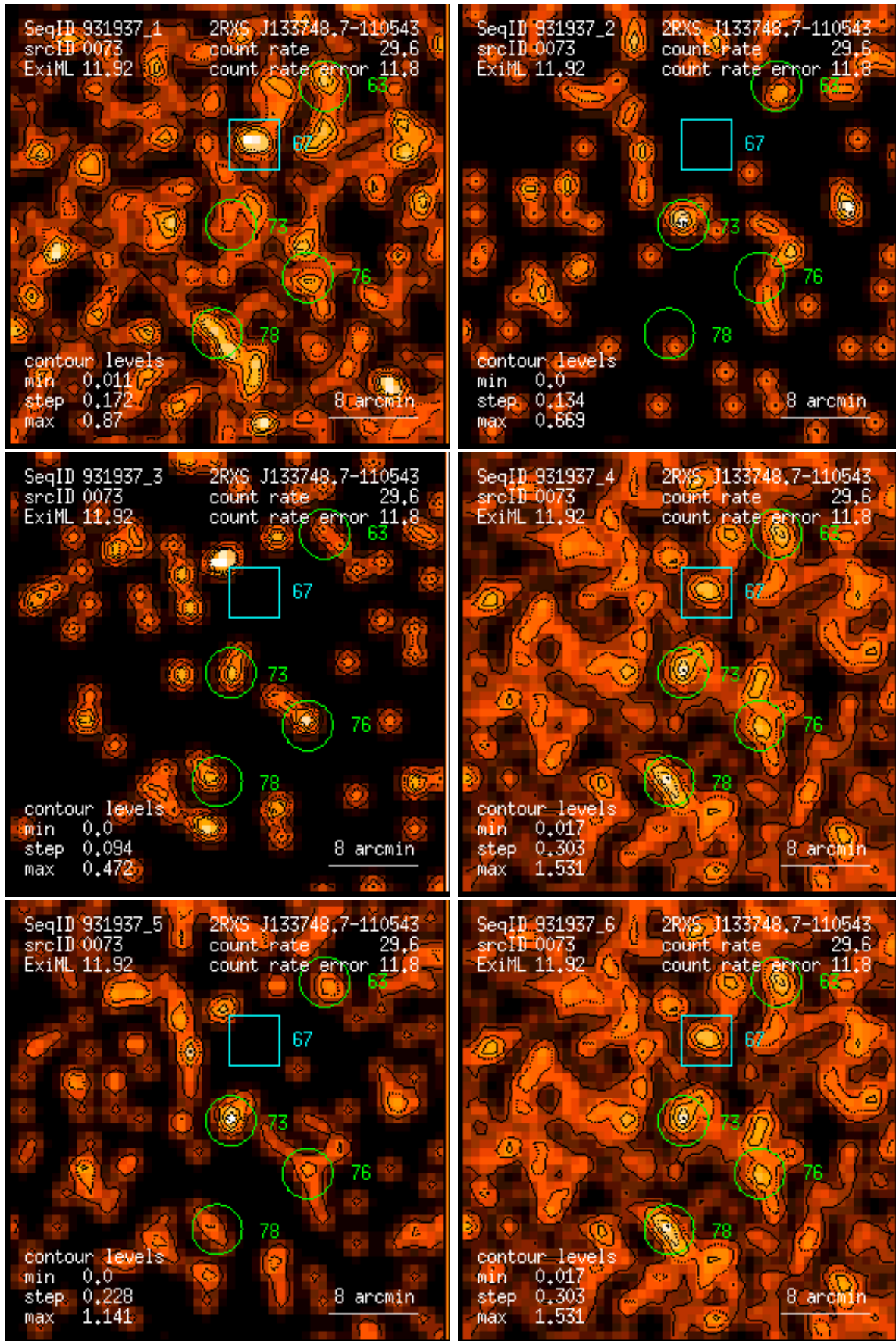
Figure 73: RASS 931937: detection 0073: band rate images, Gaussian filter: (1) PSPC channels 11 – 41, (2) 52 – 90, (3) 91 – 201, (4) 11 – 235, (5) 52 – 201, (6) 11 – 201. Broad band rates in counts/ks. Band rate contour levels in counts/ks/arcmin 2 .
