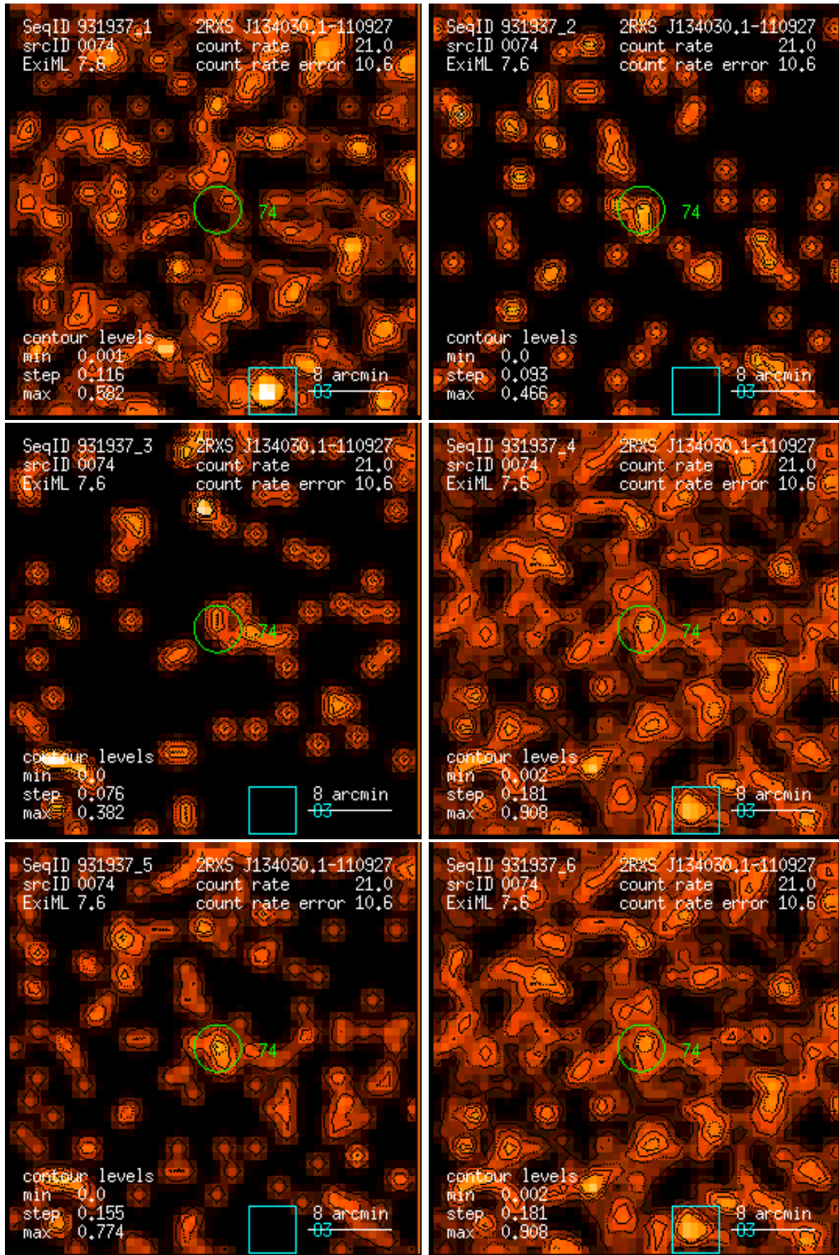
Figure 74: RASS 931937: detection 0074: band rate images, Gaussian filter: (1) PSPC channels 11 – 41, (2) 52 – 90, (3) 91 – 201, (4) 11 – 235, (5) 52 – 201, (6) 11 – 201. Broad band rates in counts/ks. Band rate contour levels in counts/ks/arcmin 2 .
