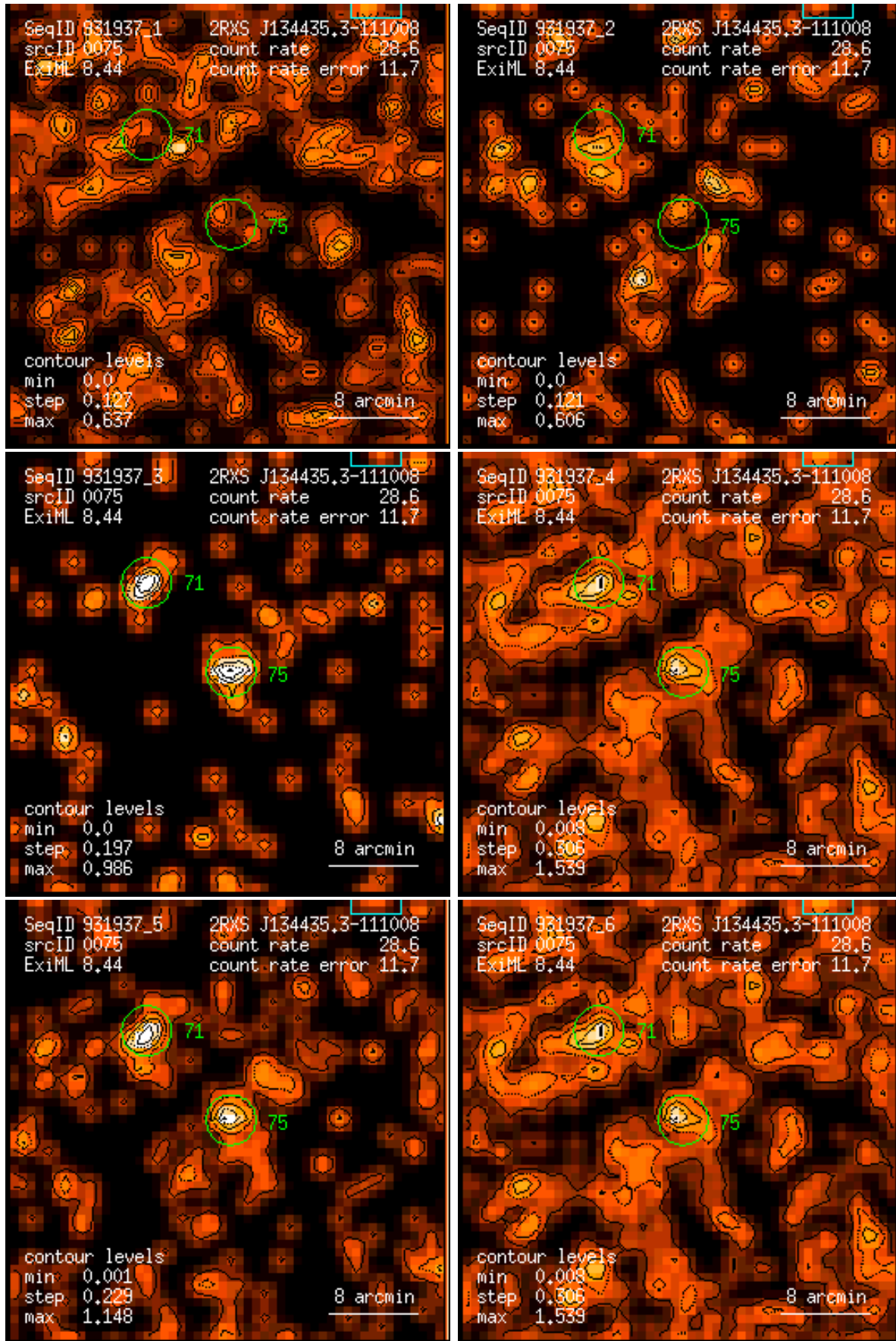
Figure 75: RASS 931937: detection 0075: band rate images, Gaussian filter: (1) PSPC channels 11 – 41, (2) 52 – 90, (3) 91 – 201, (4) 11 – 235, (5) 52 – 201, (6) 11 – 201. Broad band rates in counts/ks. Band rate contour levels in counts/ks/arcmin 2 .
