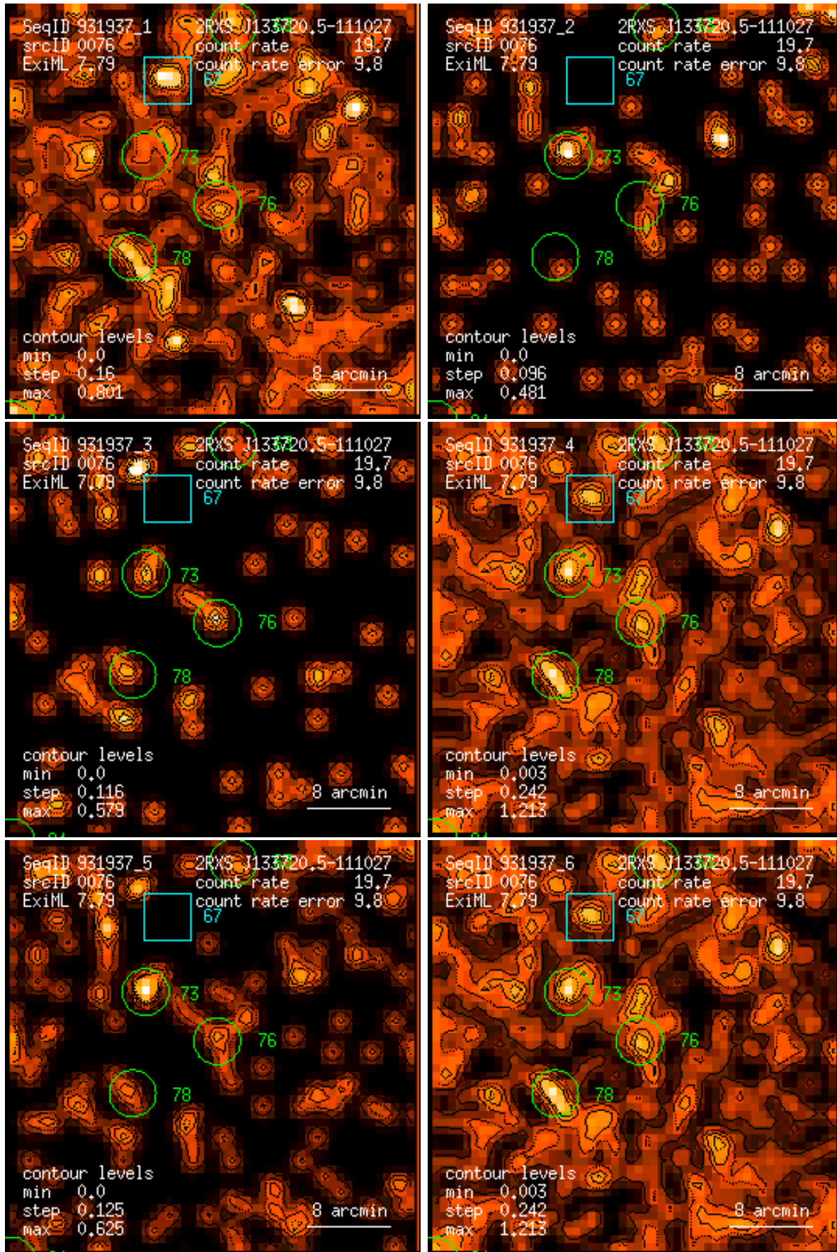
Figure 76: RASS 931937: detection 0076: band rate images, Gaussian filter: (1) PSPC channels 11 – 41, (2) 52 – 90, (3) 91 – 201, (4) 11 – 235, (5) 52 – 201, (6) 11 – 201. Broad band rates in counts/ks. Band rate contour levels in counts/ks/arcmin 2 .
