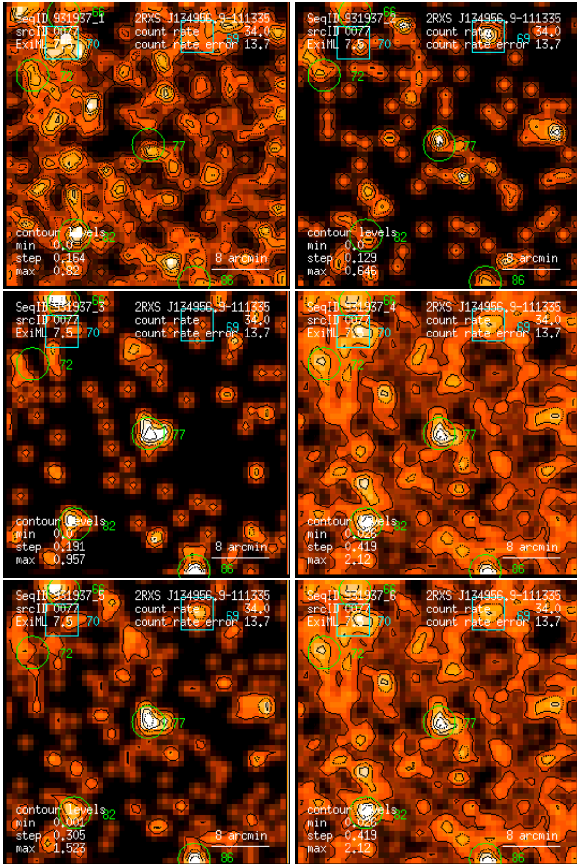
Figure 77: RASS 931937: detection 0077: band rate images, Gaussian filter: (1) PSPC channels 11 – 41, (2) 52 – 90, (3) 91 – 201, (4) 11 – 235, (5) 52 – 201, (6) 11 – 201. Broad band rates in counts/ks. Band rate contour levels in counts/ks/arcmin 2 .
