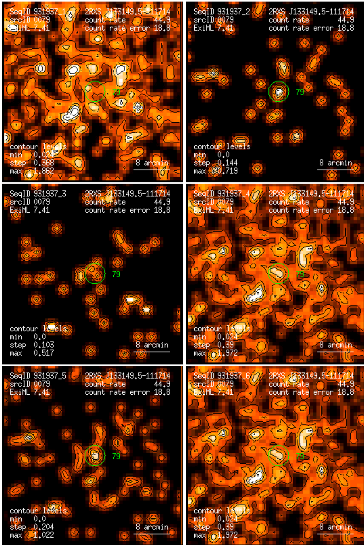
Figure 79: RASS 931937: detection 0079: band rate images, Gaussian filter: (1) PSPC channels 11 – 41, (2) 52 – 90, (3) 91 – 201, (4) 11 – 235, (5) 52 – 201, (6) 11 – 201. Broad band rates in counts/ks. Band rate contour levels in counts/ks/arcmin 2 .
