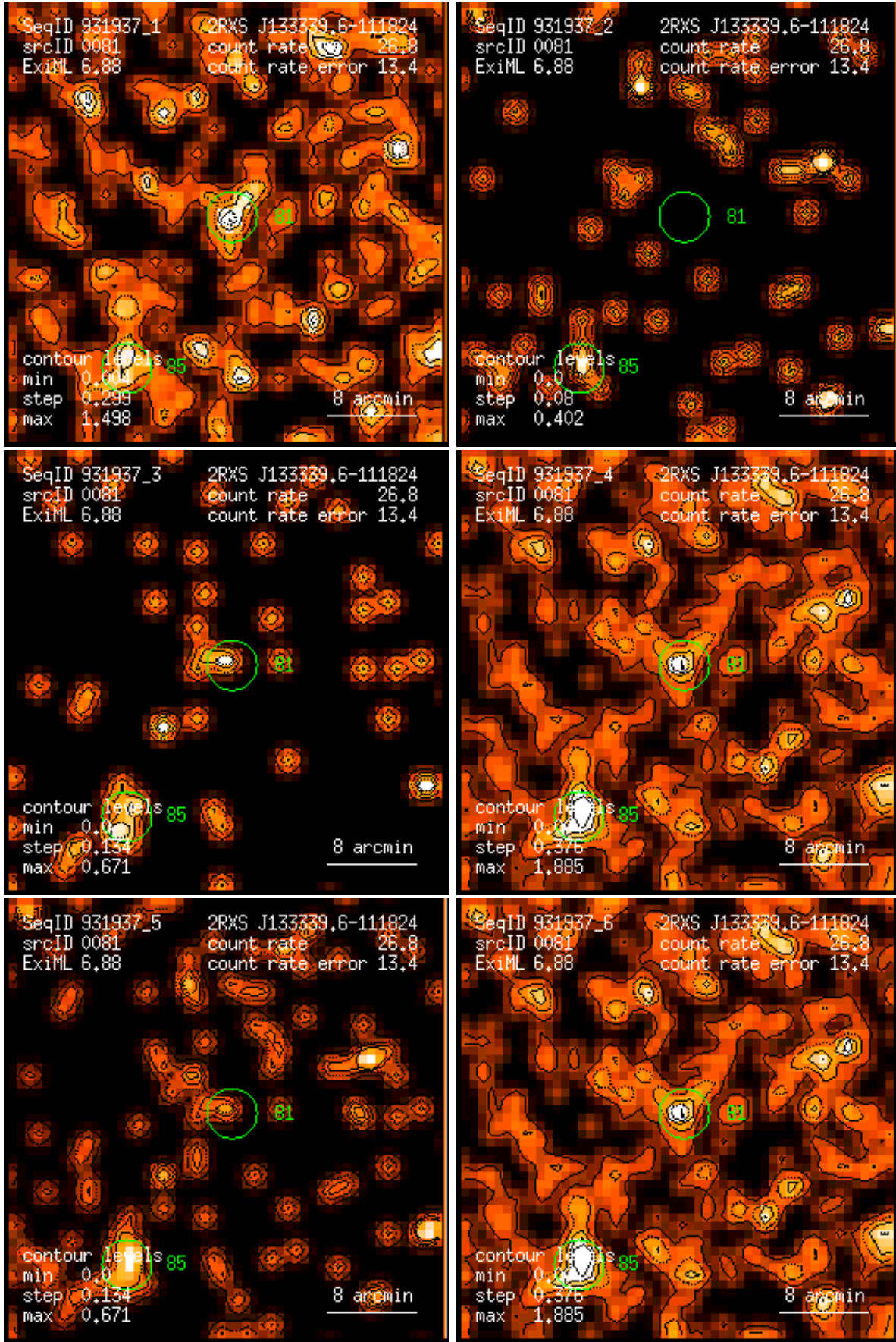
Figure 81: RASS 931937: detection 0081: band rate images, Gaussian filter: (1) PSPC channels 11 – 41, (2) 52 – 90, (3) 91 – 201, (4) 11 – 235, (5) 52 – 201, (6) 11 – 201. Broad band rates in counts/ks. Band rate contour levels in counts/ks/arcmin 2 .
