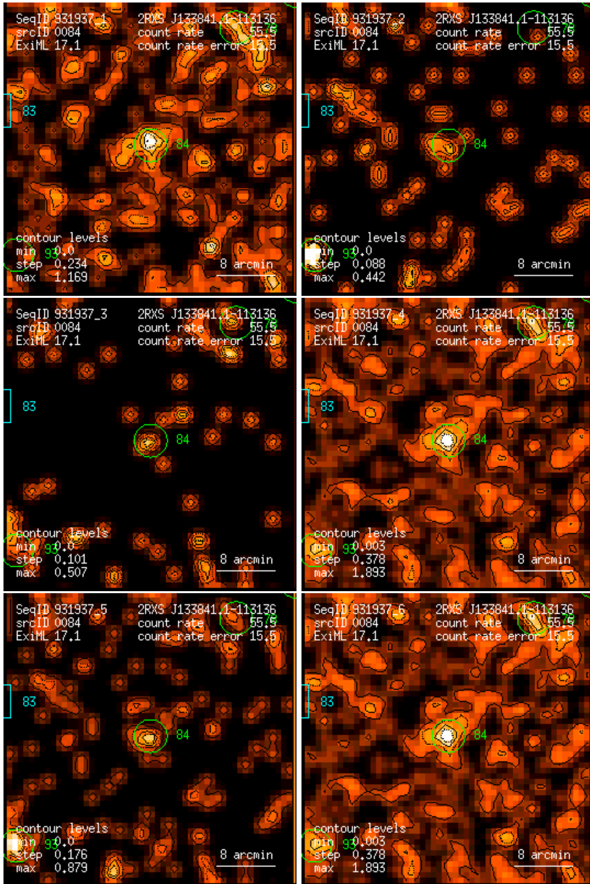
Figure 84: RASS 931937: detection 0084: band rate images, Gaussian filter: (1) PSPC channels 11 – 41, (2) 52 – 90, (3) 91 – 201, (4) 11 – 235, (5) 52 – 201, (6) 11 – 201. Broad band rates in counts/ks. Band rate contour levels in counts/ks/arcmin 2 .
