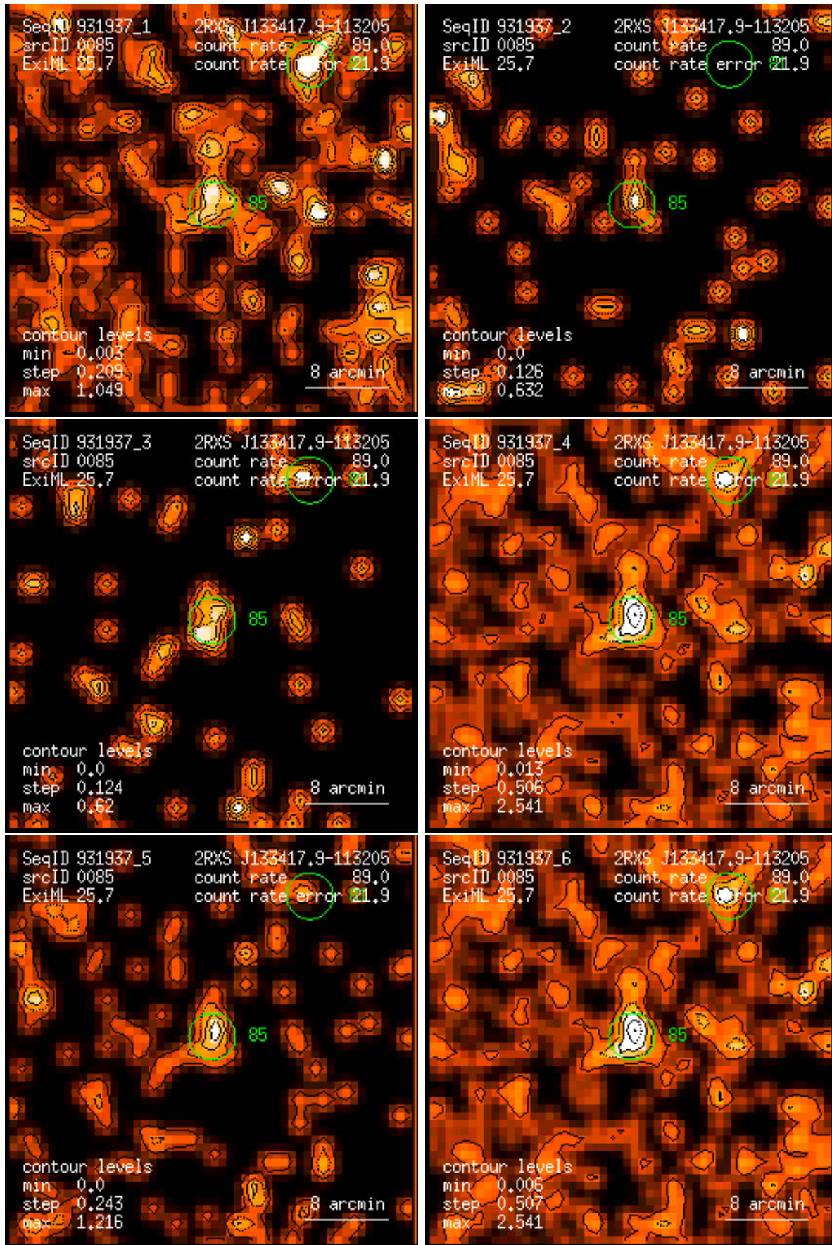
Figure 85: RASS 931937: detection 0085: band rate images, Gaussian filter: (1) PSPC channels 11 – 41, (2) 52 – 90, (3) 91 – 201, (4) 11 – 235, (5) 52 – 201, (6) 11 – 201. Broad band rates in counts/ks. Band rate contour levels in counts/ks/arcmin 2 .
