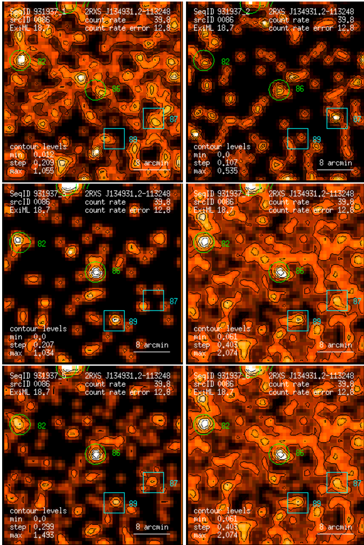
Figure 86: RASS 931937: detection 0086: band rate images, Gaussian filter: (1) PSPC channels 11 – 41, (2) 52 – 90, (3) 91 – 201, (4) 11 – 235, (5) 52 – 201, (6) 11 – 201. Broad band rates in counts/ks. Band rate contour levels in counts/ks/arcmin 2 .
