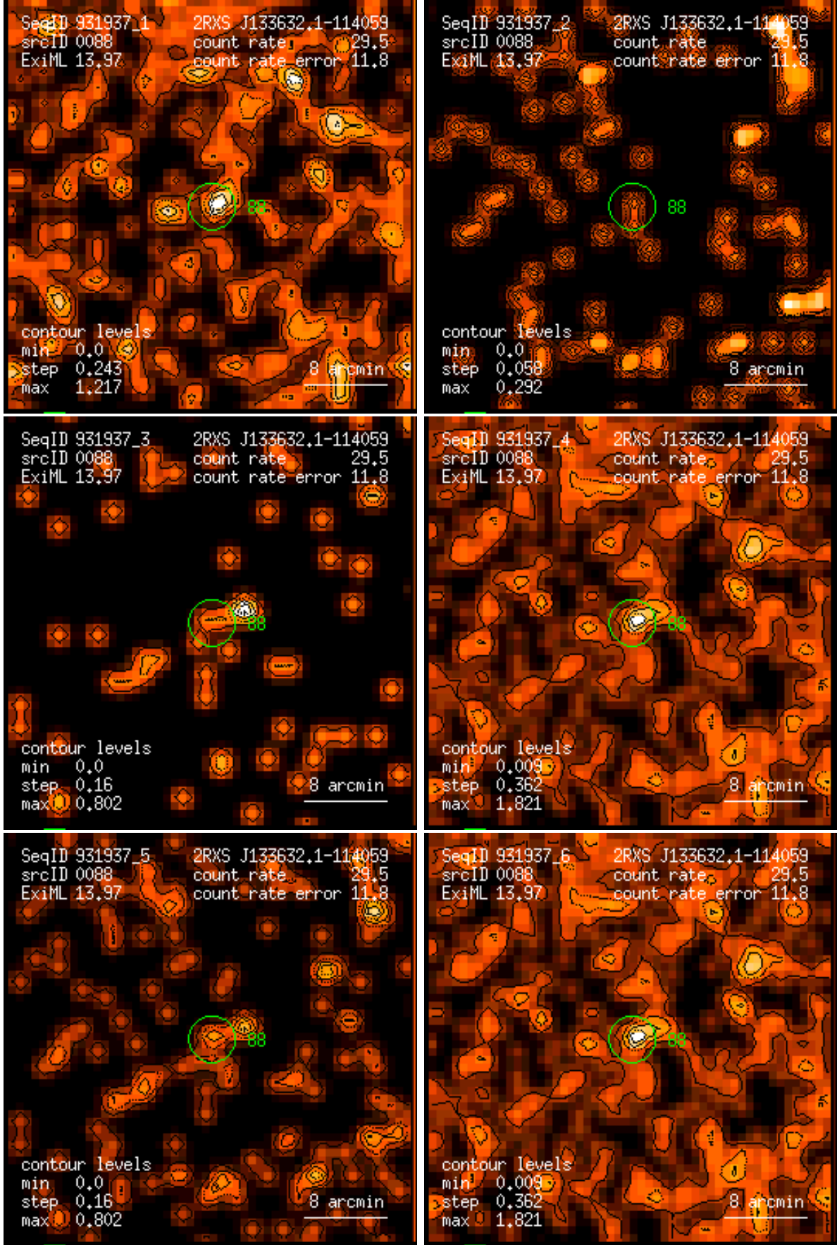
Figure 88: RASS 931937: detection 0088: band rate images, Gaussian filter: (1) PSPC channels 11 – 41, (2) 52 – 90, (3) 91 – 201, (4) 11 – 235, (5) 52 – 201, (6) 11 – 201. Broad band rates in counts/ks. Band rate contour levels in counts/ks/arcmin 2 .
