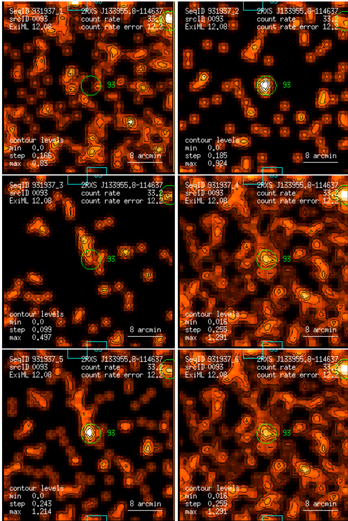
Figure 93: RASS 931937: detection 0093: band rate images, Gaussian filter: (1) PSPC channels 11 – 41, (2) 52 – 90, (3) 91 – 201, (4) 11 – 235, (5) 52 – 201, (6) 11 – 201. Broad band rates in counts/ks. Band rate contour levels in counts/ks/arcmin 2 .
