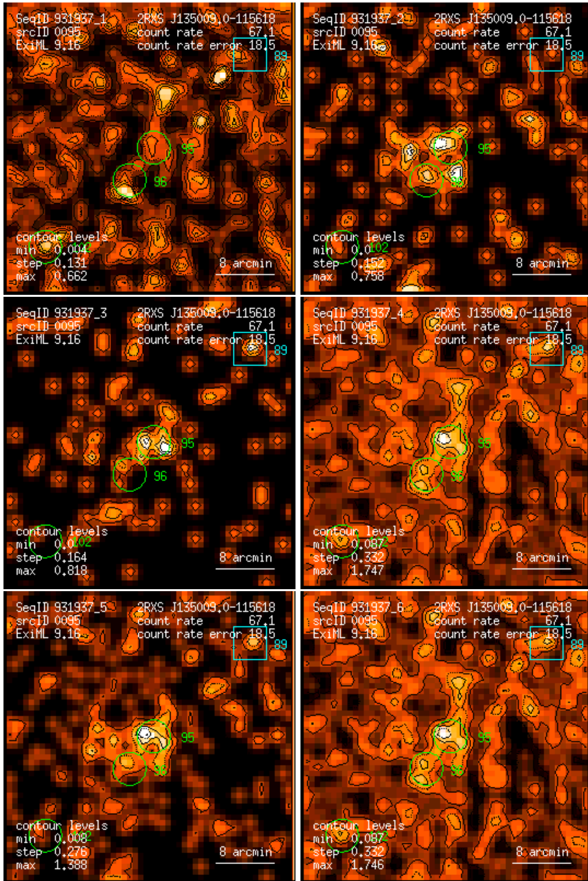
Figure 95: RASS 931937: detection 0095: band rate images, Gaussian filter: (1) PSPC channels 11 – 41, (2) 52 – 90, (3) 91 – 201, (4) 11 – 235, (5) 52 – 201, (6) 11 – 201. Broad band rates in counts/ks. Band rate contour levels in counts/ks/arcmin 2 .
