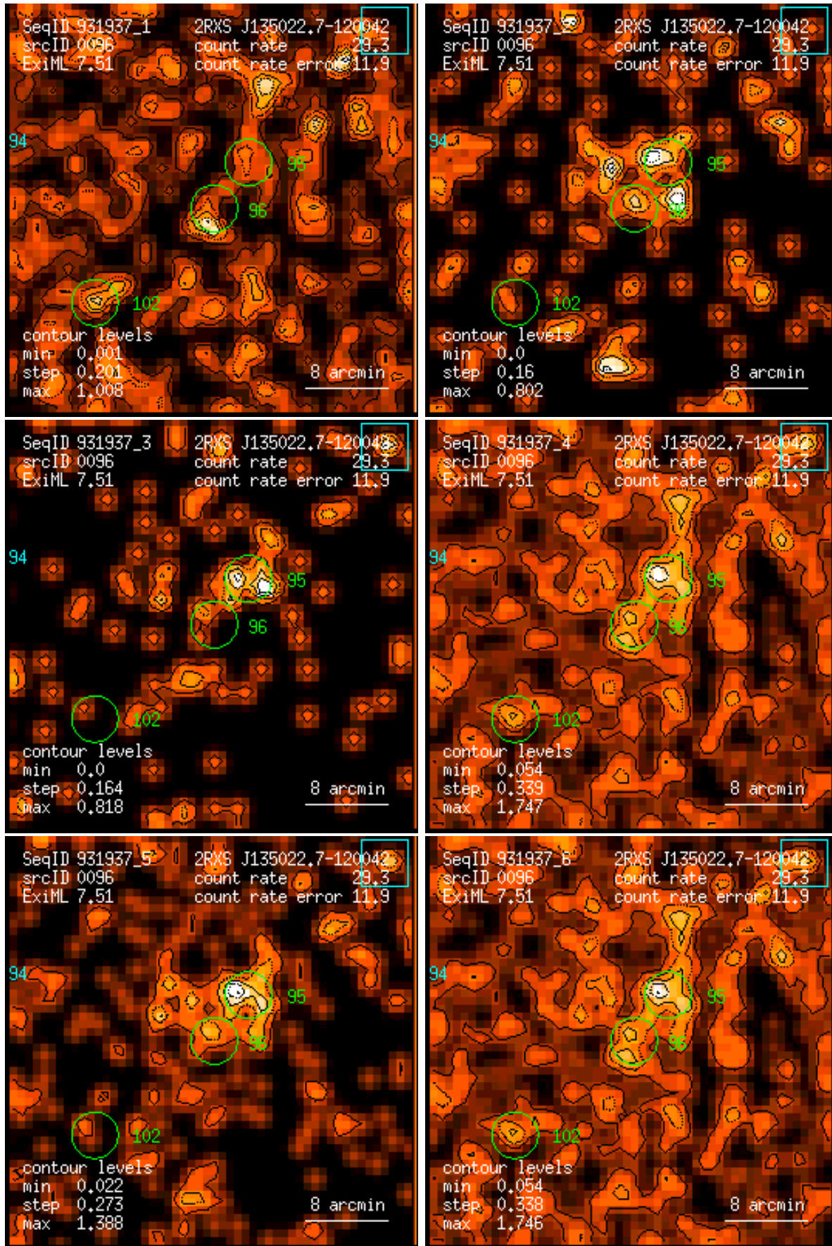
Figure 96: RASS 931937: detection 0096: band rate images, Gaussian filter: (1) PSPC channels 11 – 41, (2) 52 – 90, (3) 91 – 201, (4) 11 – 235, (5) 52 – 201, (6) 11 – 201. Broad band rates in counts/ks. Band rate contour levels in counts/ks/arcmin 2 .
