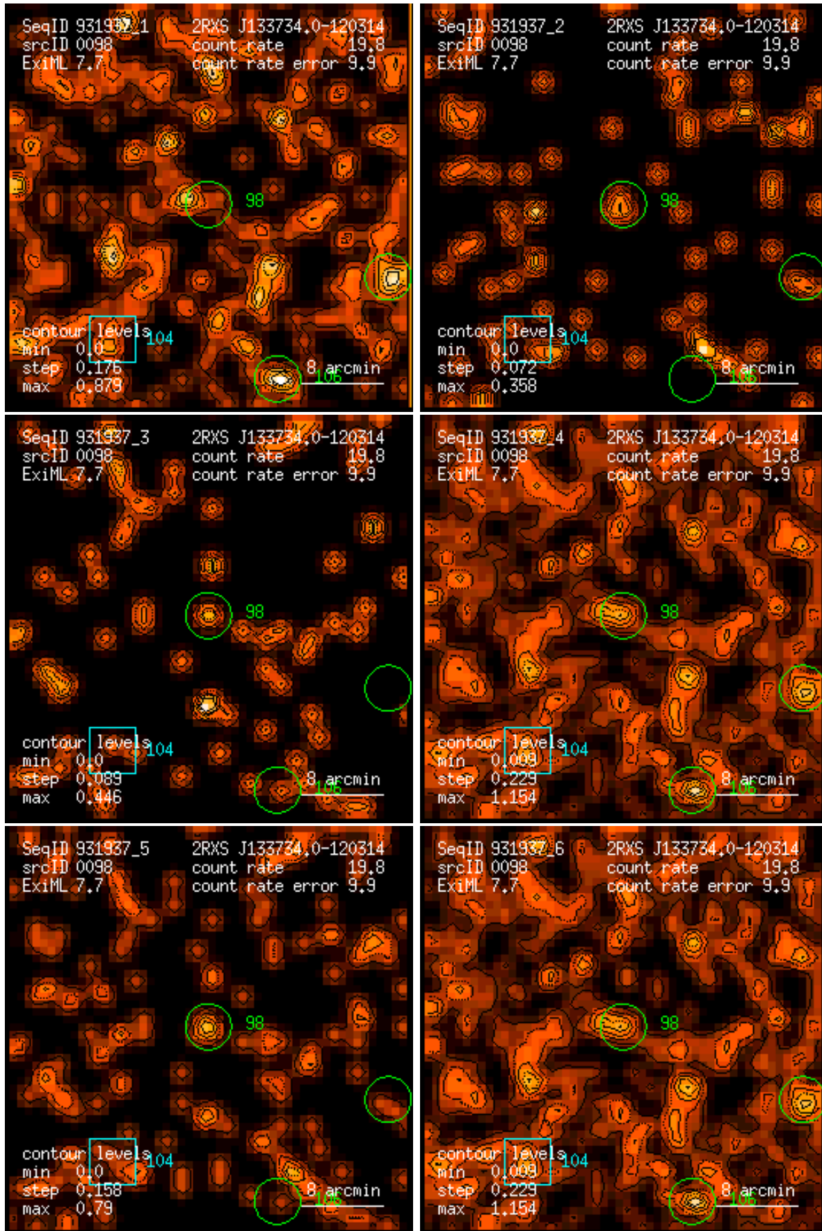
Figure 98: RASS 931937: detection 0098: band rate images, Gaussian filter: (1) PSPC channels 11 – 41, (2) 52 – 90, (3) 91 – 201, (4) 11 – 235, (5) 52 – 201, (6) 11 – 201. Broad band rates in counts/ks. Band rate contour levels in counts/ks/arcmin 2 .
