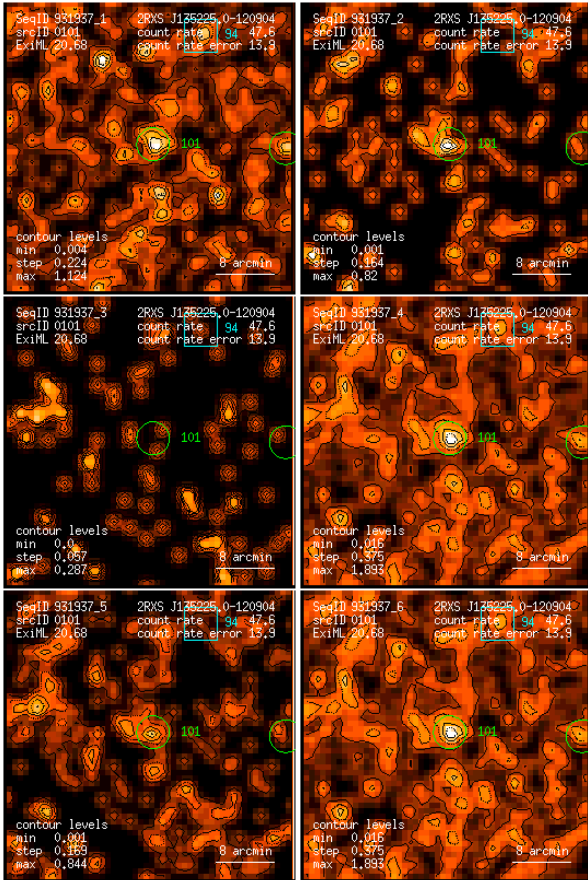
Figure 101: RASS 931937: detection 0101: band rate images, Gaussian filter: (1) PSPC channels 11 – 41, (2) 52 – 90, (3) 91 – 201, (4) 11 – 235, (5) 52 – 201, (6) 11 – 201. Broad band rates in counts/ks. Band rate contour levels in counts/ks/arcmin 2 .
