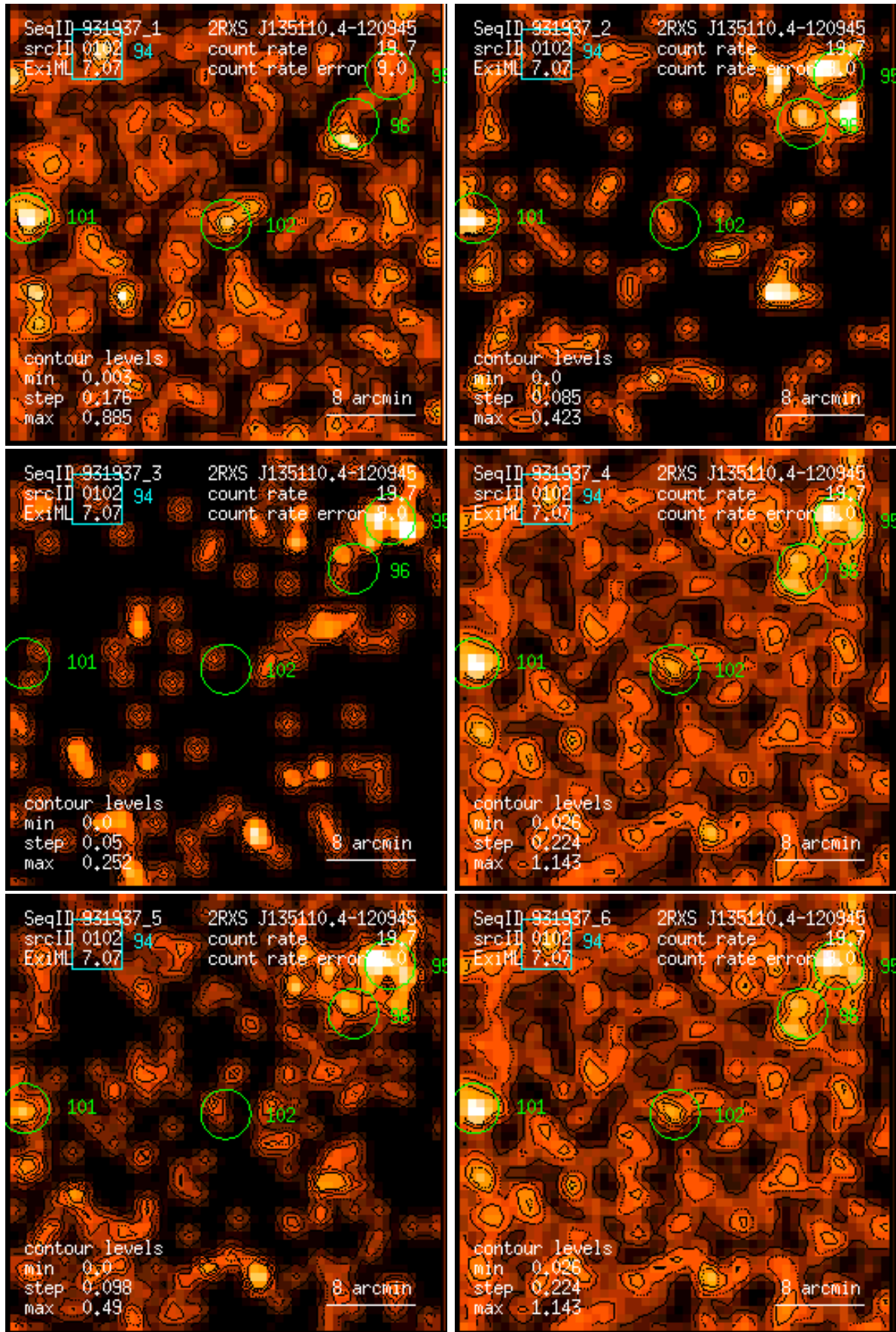
Figure 102: RASS 931937: detection 0102: band rate images, Gaussian filter: (1) PSPC channels 11 – 41, (2) 52 – 90, (3) 91 – 201, (4) 11 – 235, (5) 52 – 201, (6) 11 – 201. Broad band rates in counts/ks. Band rate contour levels in counts/ks/arcmin 2 .
