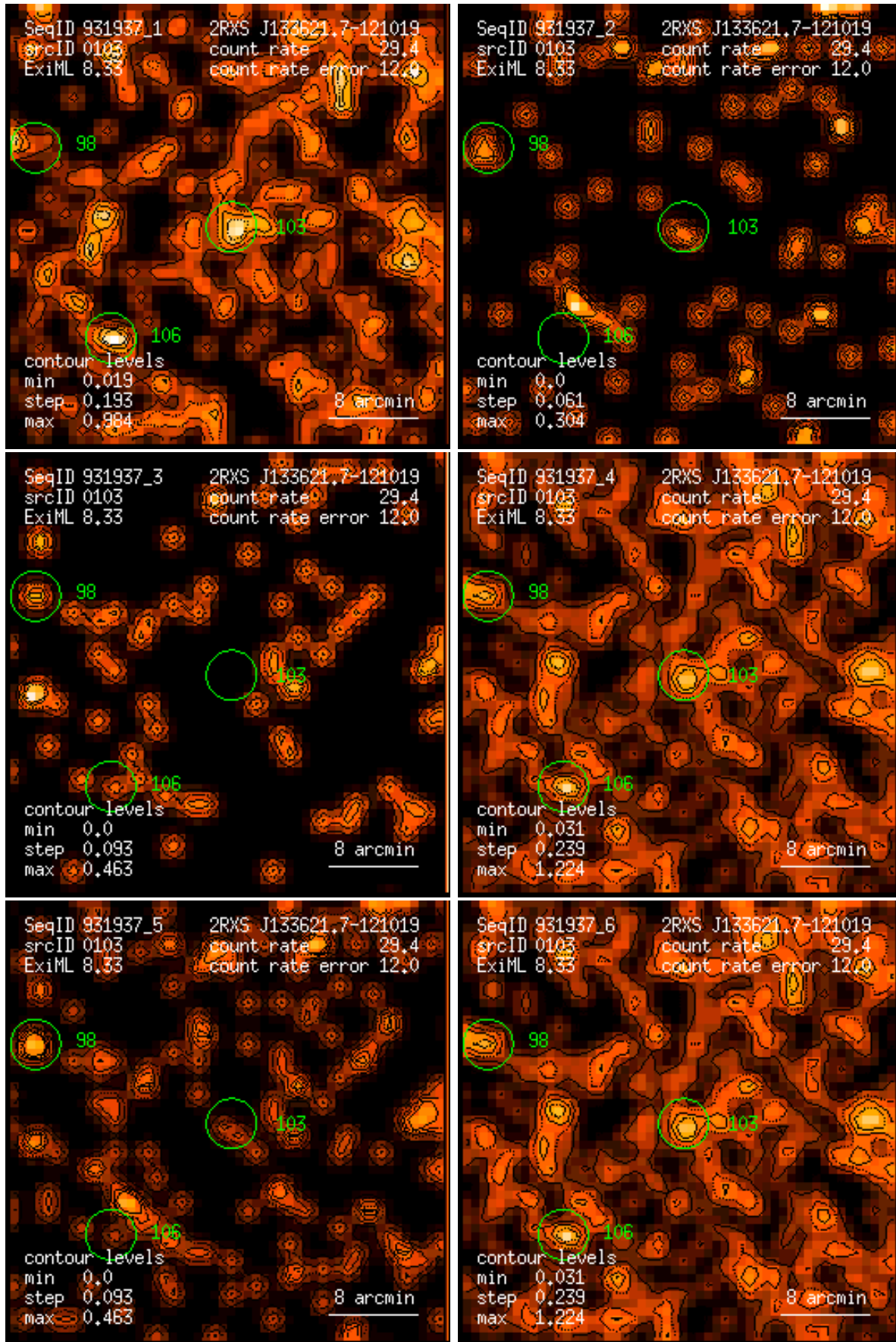
Figure 103: RASS 931937: detection 0103: band rate images, Gaussian filter: (1) PSPC channels 11 – 41, (2) 52 – 90, (3) 91 – 201, (4) 11 – 235, (5) 52 – 201, (6) 11 – 201. Broad band rates in counts/ks. Band rate contour levels in counts/ks/arcmin 2 .
