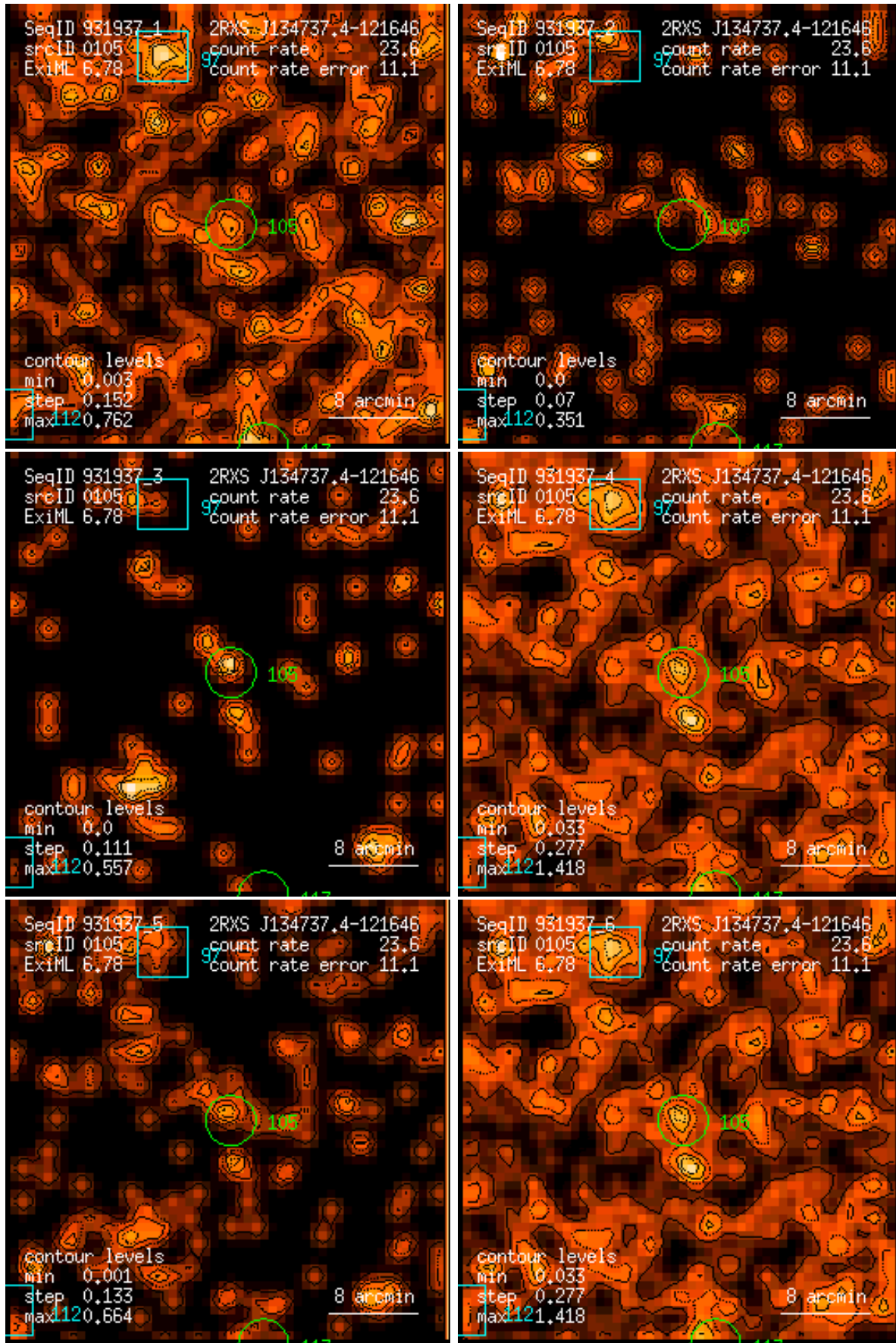
Figure 105: RASS 931937: detection 0105: band rate images, Gaussian filter: (1) PSPC channels 11 – 41, (2) 52 – 90, (3) 91 – 201, (4) 11 – 235, (5) 52 – 201, (6) 11 – 201. Broad band rates in counts/ks. Band rate contour levels in counts/ks/arcmin 2 .
