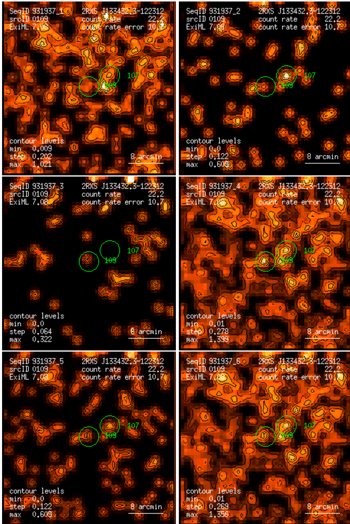
Figure 109: RASS 931937: detection 0109: band rate images, Gaussian filter: (1) PSPC channels 11 – 41, (2) 52 – 90, (3) 91 – 201, (4) 11 – 235, (5) 52 – 201, (6) 11 – 201. Broad band rates in counts/ks. Band rate contour levels in counts/ks/arcmin 2 .
