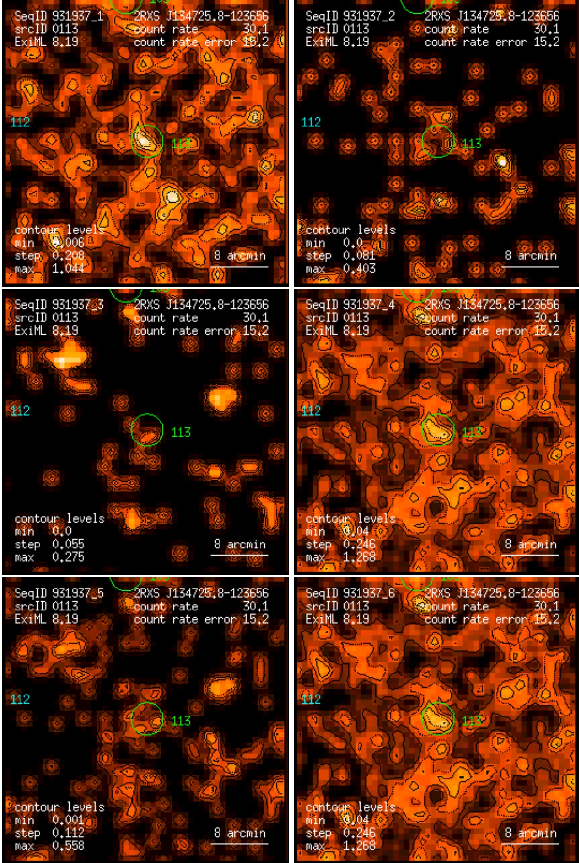
Figure 113: RASS 931937: detection 0113: band rate images, Gaussian filter: (1) PSPC channels 11 – 41, (2) 52 – 90, (3) 91 – 201, (4) 11 – 235, (5) 52 – 201, (6) 11 – 201. Broad band rates in counts/ks. Band rate contour levels in counts/ks/arcmin 2 .
