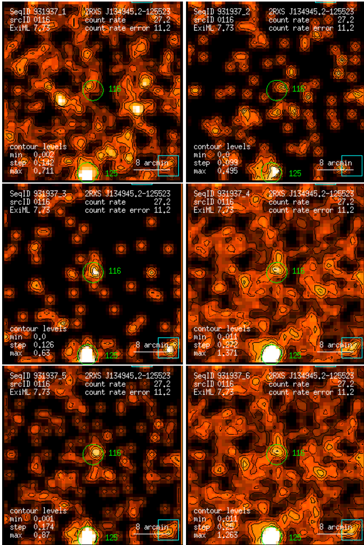
Figure 116: RASS 931937: detection 0116: band rate images, Gaussian filter: (1) PSPC channels 11 – 41, (2) 52 – 90, (3) 91 – 201, (4) 11 – 235, (5) 52 – 201, (6) 11 – 201. Broad band rates in counts/ks. Band rate contour levels in counts/ks/arcmin 2 .
