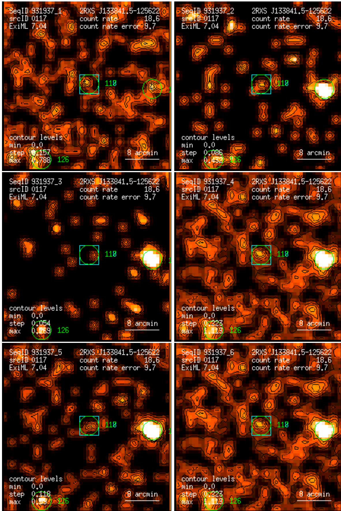
Figure 117: RASS 931937: detection 0117: band rate images, Gaussian filter: (1) PSPC channels 11 – 41, (2) 52 – 90, (3) 91 – 201, (4) 11 – 235, (5) 52 – 201, (6) 11 – 201. Broad band rates in counts/ks. Band rate contour levels in counts/ks/arcmin 2 .
