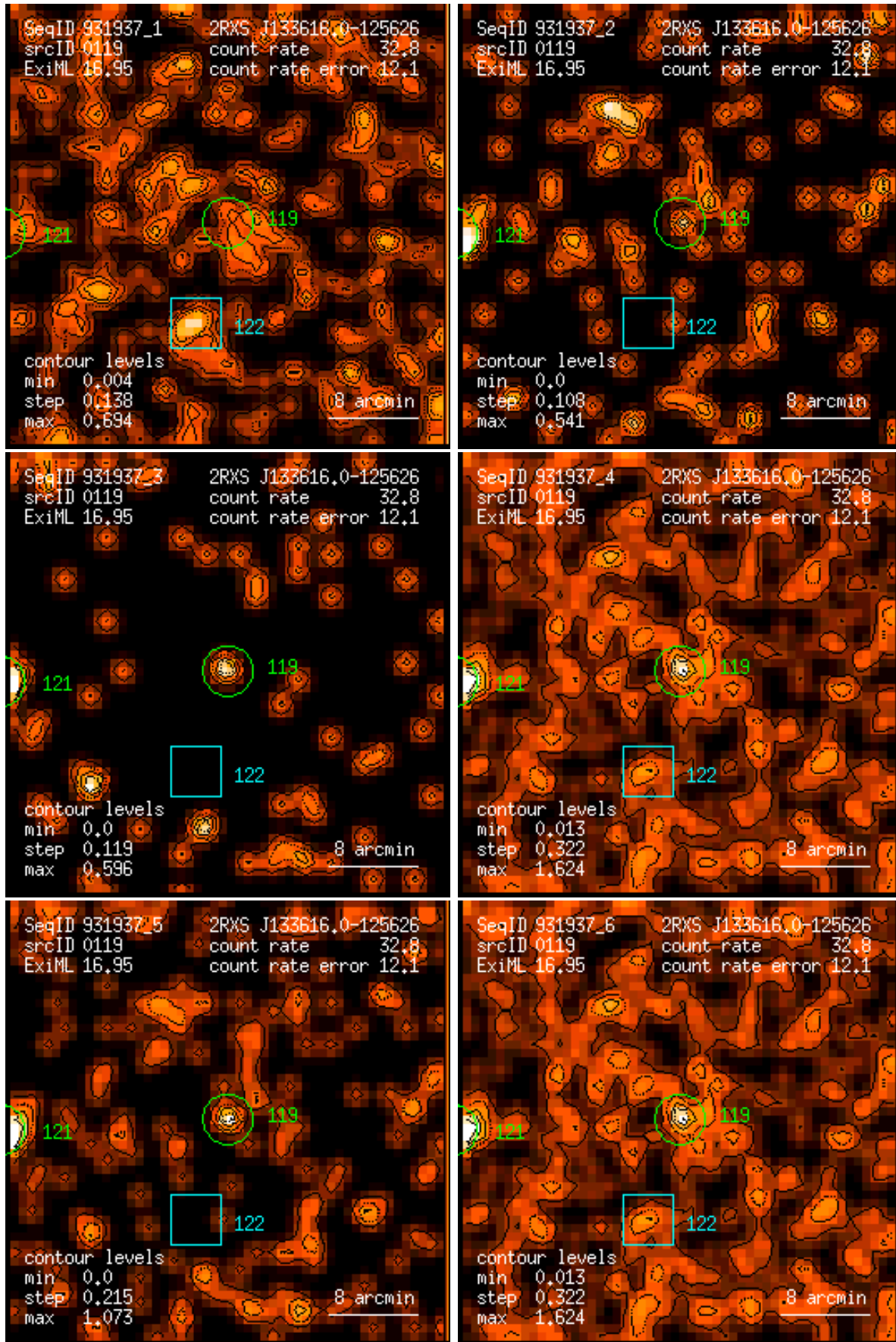
Figure 119: RASS 931937: detection 0119: band rate images, Gaussian filter: (1) PSPC channels 11 – 41, (2) 52 – 90, (3) 91 – 201, (4) 11 – 235, (5) 52 – 201, (6) 11 – 201. Broad band rates in counts/ks. Band rate contour levels in counts/ks/arcmin 2 .
