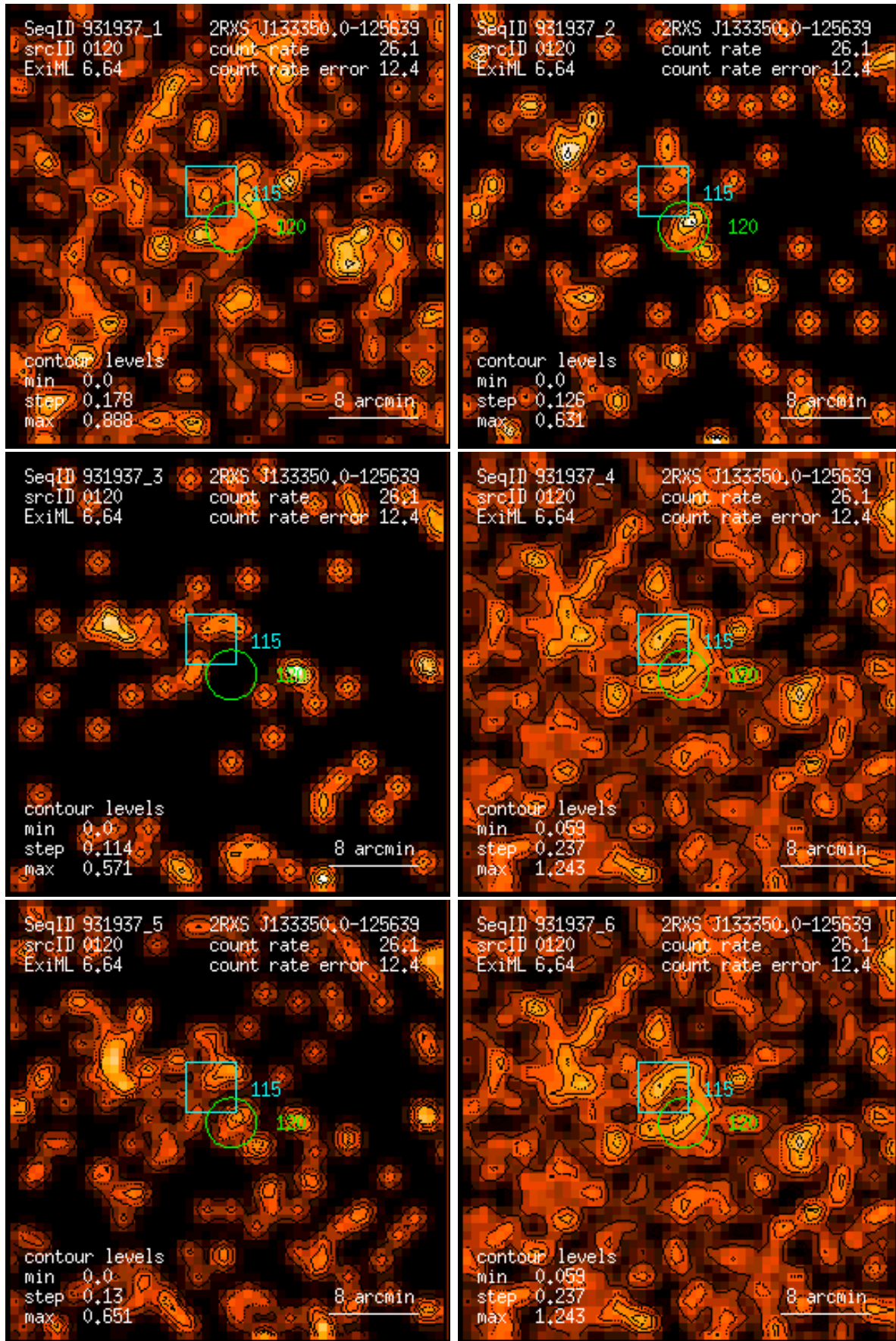
Figure 120: RASS 931937: detection 0120: band rate images, Gaussian filter: (1) PSPC channels 11 – 41, (2) 52 – 90, (3) 91 – 201, (4) 11 – 235, (5) 52 – 201, (6) 11 – 201. Broad band rates in counts/ks. Band rate contour levels in counts/ks/arcmin 2 .
