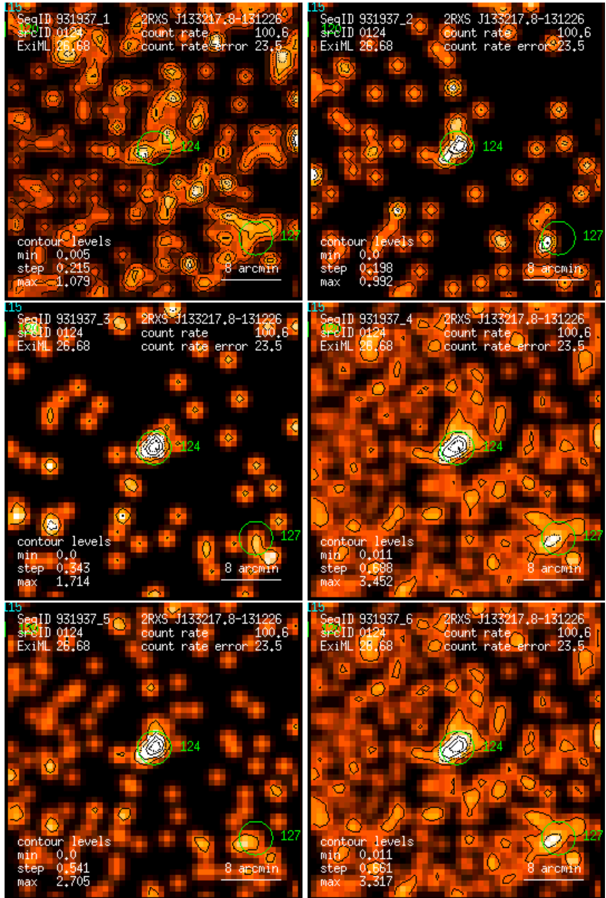
Figure 124: RASS 931937: detection 0124: band rate images, Gaussian filter: (1) PSPC channels 11 – 41, (2) 52 – 90, (3) 91 – 201, (4) 11 – 235, (5) 52 – 201, (6) 11 – 201. Broad band rates in counts/ks. Band rate contour levels in counts/ks/arcmin 2 .
