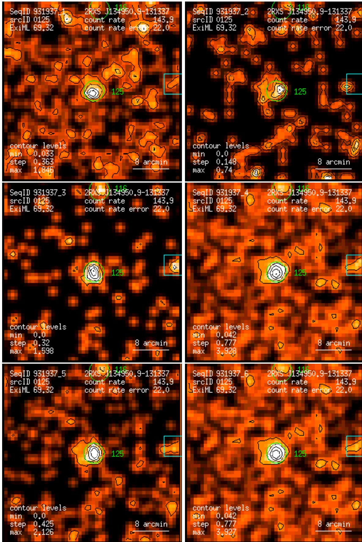
Figure 125: RASS 931937: detection 0125: band rate images, Gaussian filter: (1) PSPC channels 11 – 41, (2) 52 – 90, (3) 91 – 201, (4) 11 – 235, (5) 52 – 201, (6) 11 – 201. Broad band rates in counts/ks. Band rate contour levels in counts/ks/arcmin 2 .
