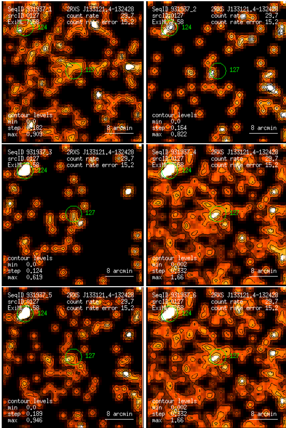
Figure 127: RASS 931937: detection 0127: band rate images, Gaussian filter: (1) PSPC channels 11 – 41, (2) 52 – 90, (3) 91 – 201, (4) 11 – 235, (5) 52 – 201, (6) 11 – 201. Broad band rates in counts/ks. Band rate contour levels in counts/ks/arcmin 2 .
