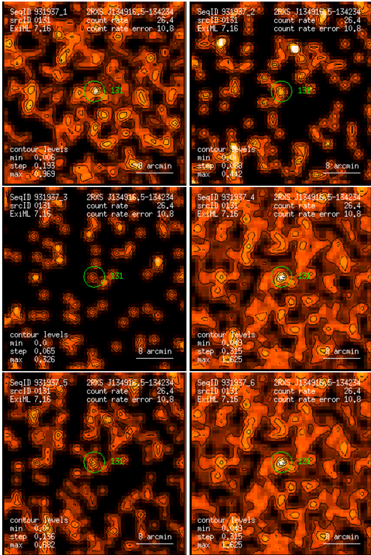
Figure 131: RASS 931937: detection 0131: band rate images, Gaussian filter: (1) PSPC channels 11 – 41, (2) 52 – 90, (3) 91 – 201, (4) 11 – 235, (5) 52 – 201, (6) 11 – 201. Broad band rates in counts/ks. Band rate contour levels in counts/ks/arcmin 2 .
