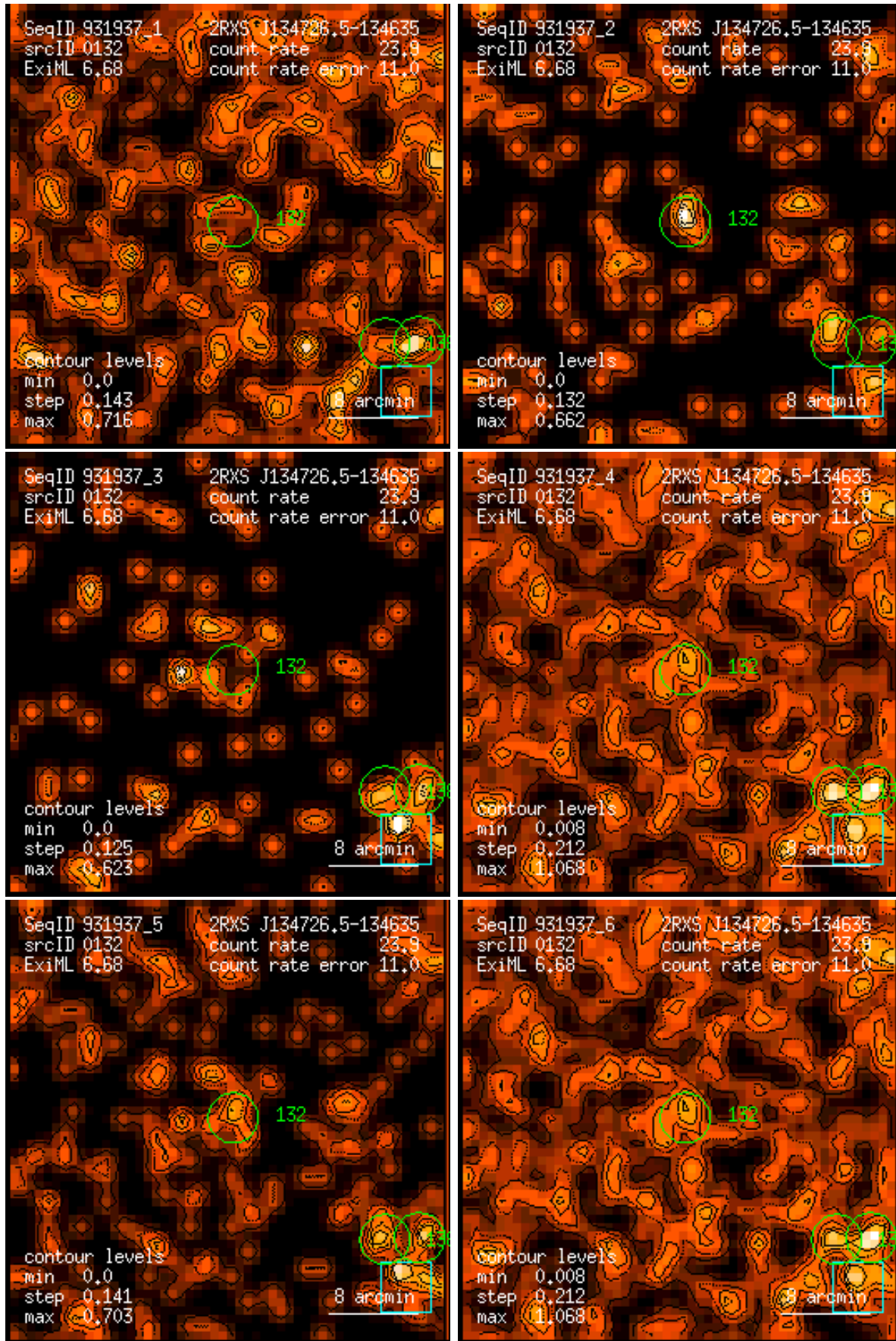
Figure 132: RASS 931937: detection 0132: band rate images, Gaussian filter: (1) PSPC channels 11 – 41, (2) 52 – 90, (3) 91 – 201, (4) 11 – 235, (5) 52 – 201, (6) 11 – 201. Broad band rates in counts/ks. Band rate contour levels in counts/ks/arcmin 2 .
