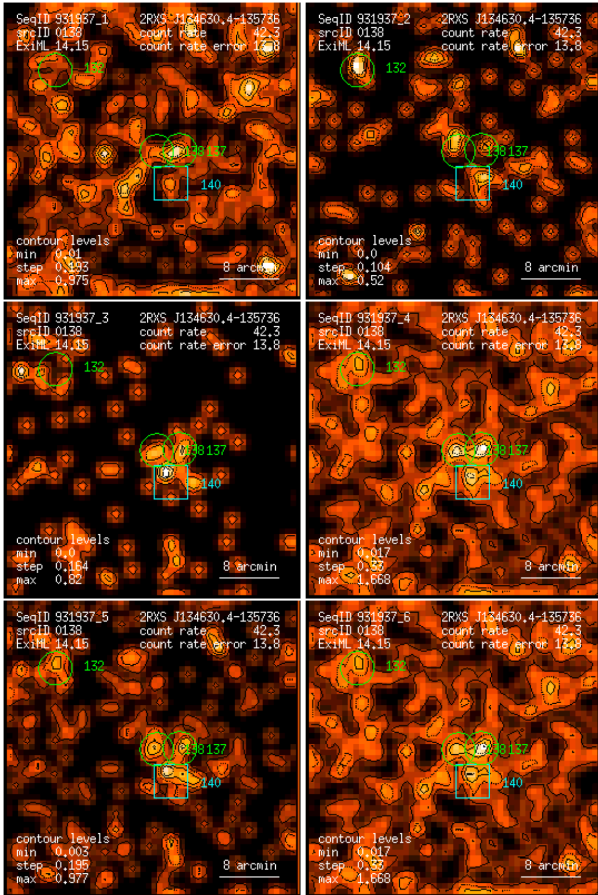
Figure 138: RASS 931937: detection 0138: band rate images, Gaussian filter: (1) PSPC channels 11 – 41, (2) 52 – 90, (3) 91 – 201, (4) 11 – 235, (5) 52 – 201, (6) 11 – 201. Broad band rates in counts/ks. Band rate contour levels in counts/ks/arcmin 2 .
