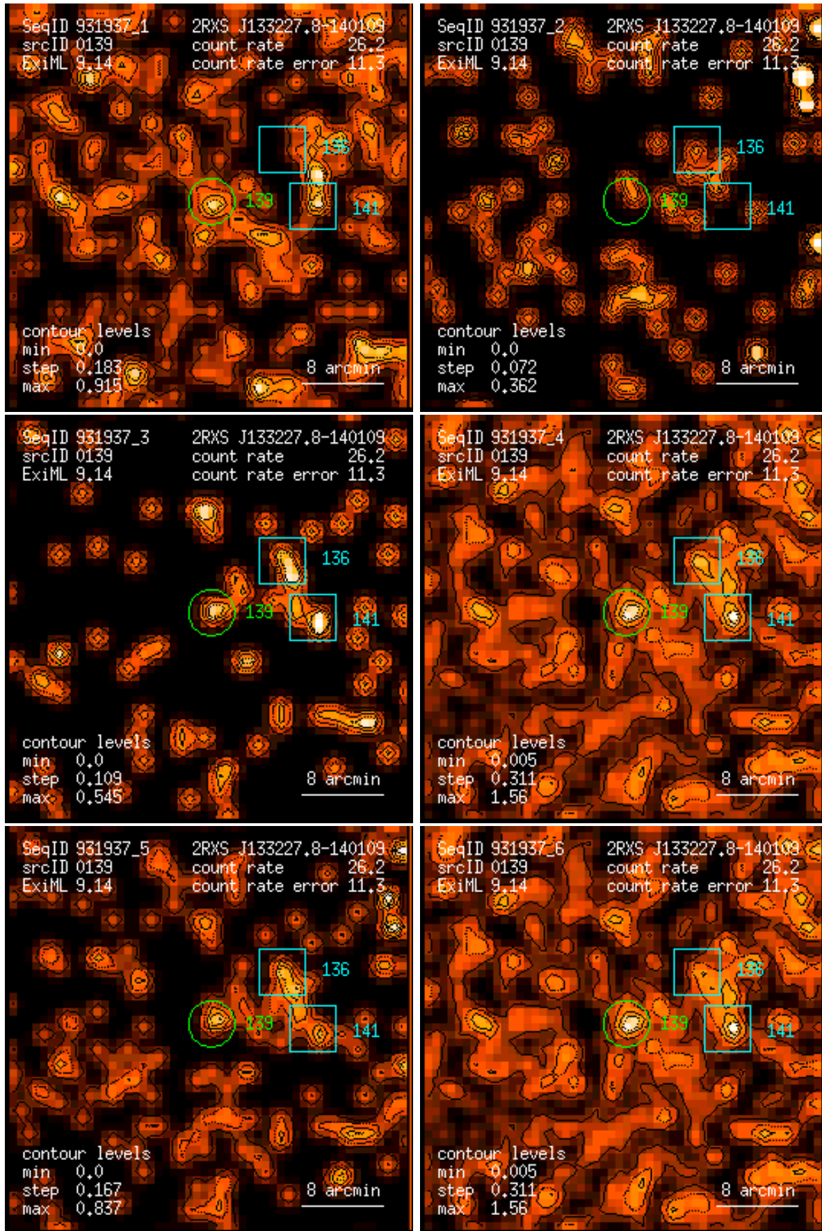
Figure 139: RASS 931937: detection 0139: band rate images, Gaussian filter: (1) PSPC channels 11 – 41, (2) 52 – 90, (3) 91 – 201, (4) 11 – 235, (5) 52 – 201, (6) 11 – 201. Broad band rates in counts/ks. Band rate contour levels in counts/ks/arcmin 2 .
